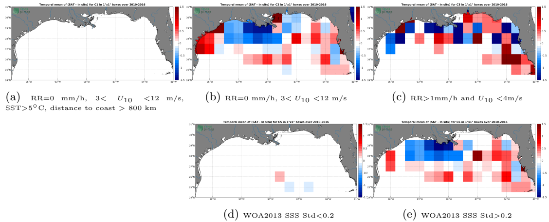
Figure 12: Temporal mean gridded over spatial boxes of size 1^\circ \times 1^\circ of \Delta SSS (SMOS-L3-BEC-OA-V1-9DAYS-0.25DEG - TSG-SAMOS) for 5 different subdatasets corresponding to:RR=0 mm/h, 3 < U_{10} < 12 m/s, SST >5^\circ C, distance to coast > 800 km (a), RR=0 mm/h, 3 < U_{10} < 12 m/s (b), RR >1 mm/h and U_{10} < 4 m/s (c), WOA2013 SSS Std <0.2 (d), WOA2013 SSS Std >0.2 (e).
