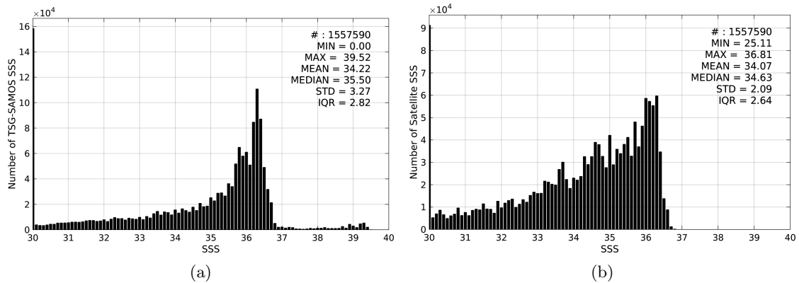
Figure 2: Histograms of SSS from TSG-SAMOS (a) and SMOS-L3-BEC-OA-V1-9DAYS-0.25DEG (b) considering all match-up pairs per bins of 0.1 over the Mississippi river plume Pi-MEP region and for the full satellite product period.
