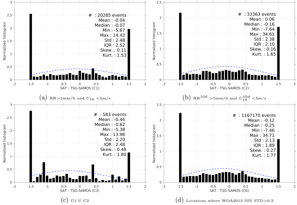
Figure 13: Normalized histogram of \Delta\text{SSS} (SMOS-L3-BEC-OA-V1-9DAYS-0.25DEG - TSG-SAMOS) for 6 different subdatasets corresponding to: RR > 1mm/h and U_{10} < 5\text{m/s} (a), \text{RR}^{10d} > 5\text{mm/h} and U_{10}^{10d} < 5\text{m/s} (b), C1 U C2 (c), Locations where WOA2013 SSS STD > 0.2 (d).
