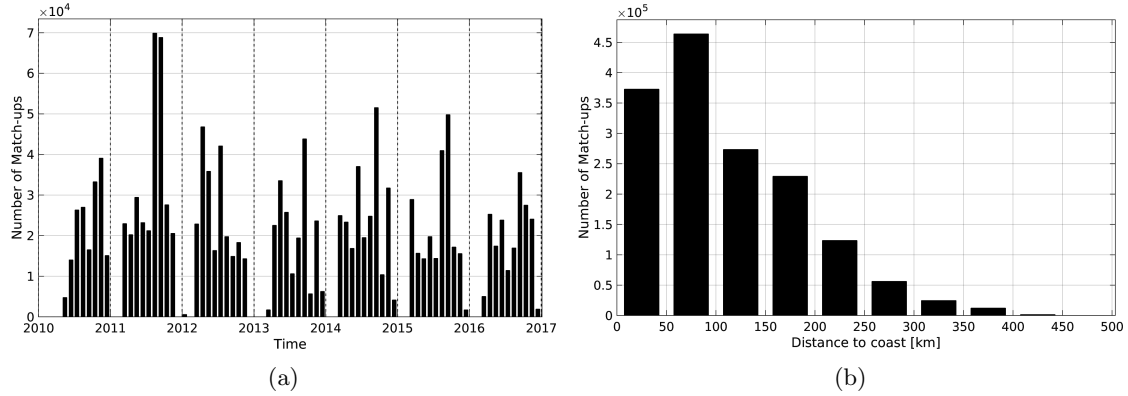
Figure 1: Number of match-ups between TSG-SAMOS and SMOS-L3-BEC-OA-V1-9DAYS-0.25DEG SSS as a function of time (a) and as function of the distance to coast (b) over the Mississippi river plume Pi-MEP region and for the full satellite product period.
