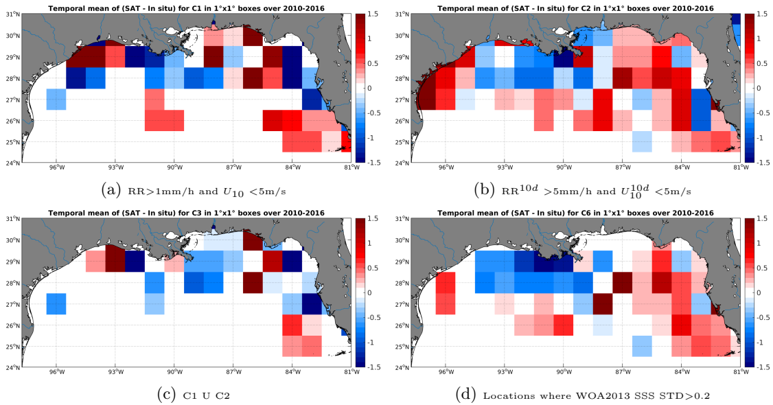
Figure 12: Temporal mean gridded over spatial boxes of size 1^\circ \times 1^\circ of \Delta SSS (SMOS-L3-BEC-OA-V1-9DAYS-0.25DEG - TSG-SAMOS) for 4 different subdatasets corresponding to:RR >1 mm/h and U_{10} <5 m/s (a), RR 10d >5 mm/h and U_{10}^{10d} <5 m/s (b), C1 U C2 (c),Locations where WOA2013 SSS STD >0.2 (d).
