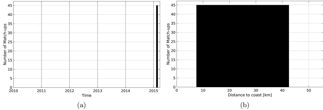
Figure 1: Number of match-ups between TSG-GOSUD-Sailing-ship and SMOS-L3-BEC-OA-V1-9DAYS-0.25DEG SSS as a function of time (a) and as function of the distance to coast (b) over the Mississippi river plume Pi-MEP region and for the full satellite product period.
