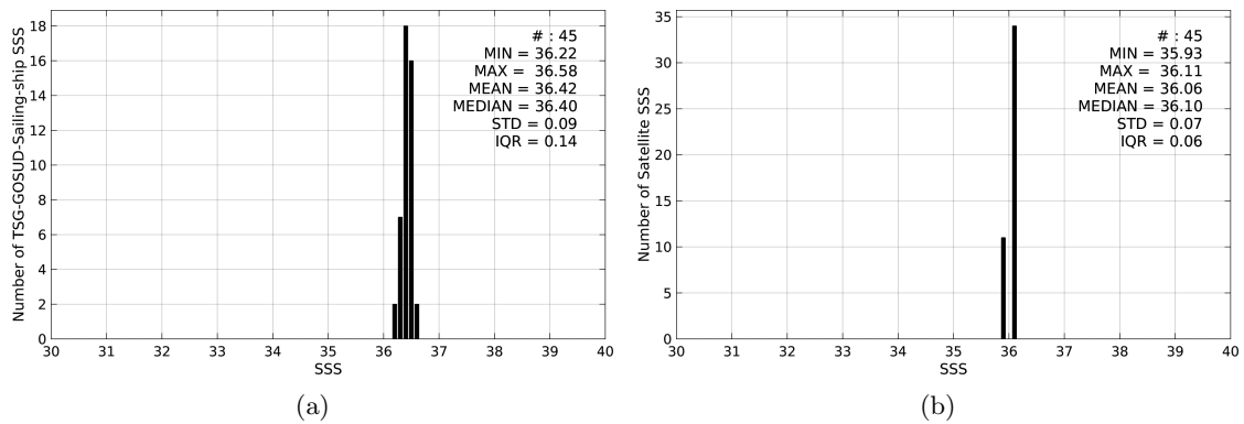
Figure 2: Histograms of SSS from TSG-GOSUD-Sailing-ship (a) and SMOS-L3-BEC-OA-V1-9DAYS-0.25DEG (b) considering all match-up pairs per bins of 0.1 over the Mississippi river plume Pi-MEP region and for the full satellite product period.
