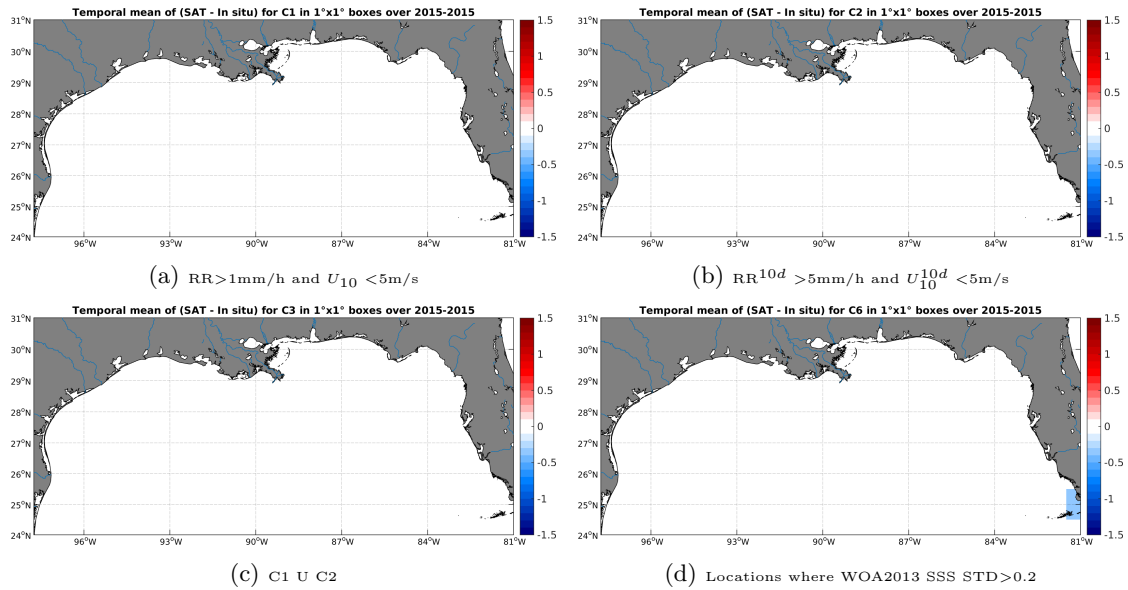
Figure 12: Temporal mean gridded over spatial boxes of size 1^\circ \times 1^\circ of \Delta SSS (SMOS-L3-BEC-OA-V1-9DAYS-0.25DEG - TSG-GOSUD-Sailing-ship) for 4 different subdatasets corresponding to:RR > 1 mm/h and U_{10} < 5 m/s (a), RR^{10d} > 5 mm/h and U_{10}^{10d} < 5 m/s (b), C1 U C2 (c),Locations where WOA2013 SSS STD > 0.2 (d).
