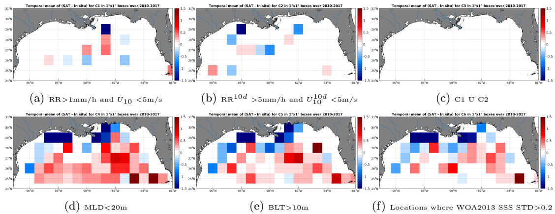
Figure 12: Temporal mean gridded over spatial boxes of size 1^\circ \times 1^\circ of \Delta SSS (SMOS-L3-BEC-OA-V1-9DAYS-0.25DEG - Argo) for 6 different subdatasets corresponding to:RR >1 mm/h and U_{10} < 5 m/s (a), RR 10d > 5 mm/h and U_{10}^{10d} < 5 m/s (b), C1 U C2 (c),MLD <20 m (d),BLT >10 m (e),Locations where WOA2013 SSS STD >0.2 (f).
