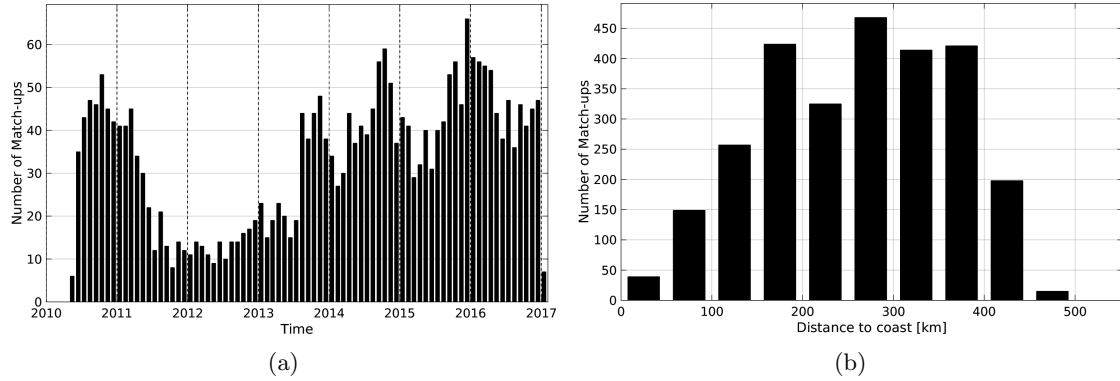
Figure 1: Number of match-ups between Argo and SMOS-L3-BEC-OA-V1-9DAYS-0.25DEG SSS as a function of time (a) and as function of the distance to coast (b) over the Mississippi river plume Pi-MEP region and for the full satellite product period.
