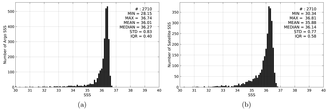
Figure 2: Histograms of SSS from Argo (a) and SMOS-L3-BEC-OA-V1-9DAYS-0.25DEG (b) considering all match-up pairs per bins of 0.1 over the Mississippi river plume Pi-MEP region and for the full satellite product period.
