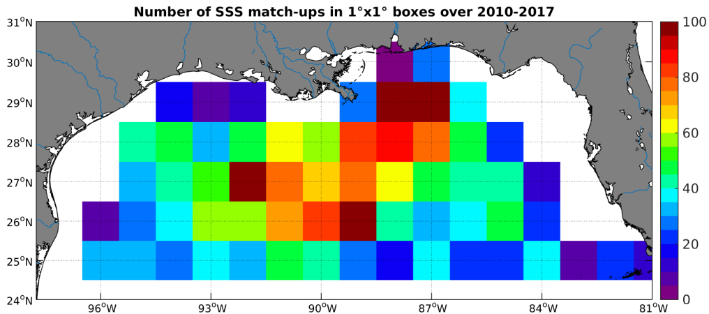
Figure 4: Number of SSS match-ups between Argo SSS and the SMOS-L3-BEC-OA-V1-9DAYS-0.25DEG SSS product for the Mississippi river plume Pi-MEP region over 1^{\circ} \times 1^{\circ} boxes and for the full satellite product period.
