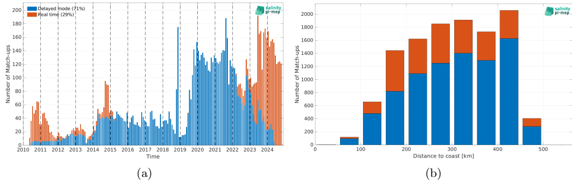
Figure 2: Number of match-ups between Argo and SMOS SSS L2-AVERAGED v700 (ESA) SSS as a function of time (a) and as function of the distance to coast (b) over the Mississippi river plume Pi-MEP region and for the full satellite product period.
