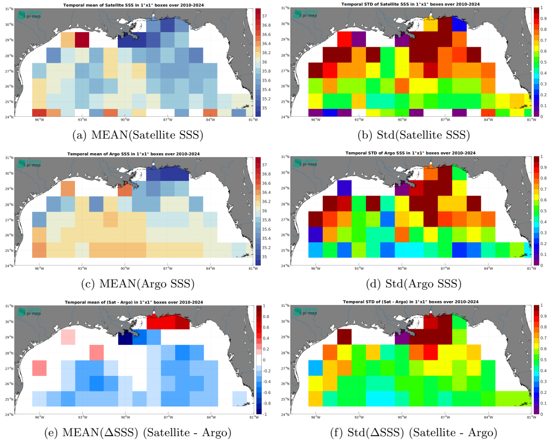
Figure 7: Temporal mean (left) and Std (right) of SSS from SMOS SSS L2-AVERAGED v700 (ESA) (top), Argo (middle), and of \Delta SSS (Satellite - Argo). Only match-up pairs are used to generate these maps.
