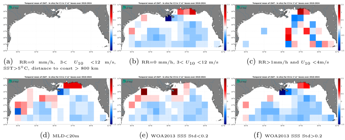
Figure 14: Temporal mean gridded over spatial boxes of size 1^\circ \times 1^\circ of \Delta SSS (SMOS SSS L2-AVERAGED v700 (ESA) - Argo) for 6 different subdatasets corresponding to:RR=0 mm/h, 3 < U_{10} < 12 m/s, SST >5^\circ C, distance to coast > 800 km (a), RR=0 mm/h, 3 < U_{10} < 12 m/s (b), RR >1 mm/h and U_{10} < 4 m/s (c),MLD <20 m (d),WOA2013 SSS Std <0.2 (e),WOA2013 SSS Std >0.2 (f).
