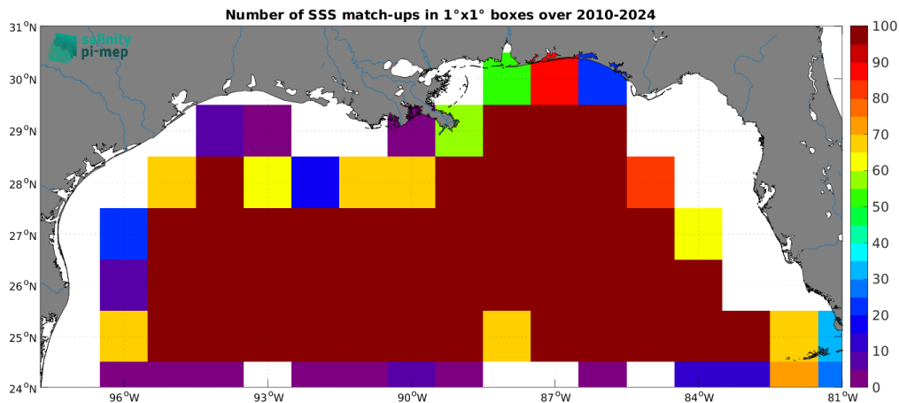
Figure 5: Number of SSS match-ups between Argo SSS and the SMOS SSS L2-AVERAGED v700 (ESA) SSS product for the Mississippi river plume Pi-MEP region over 1^\circ \times 1^\circ boxes and for the full satellite product period.
