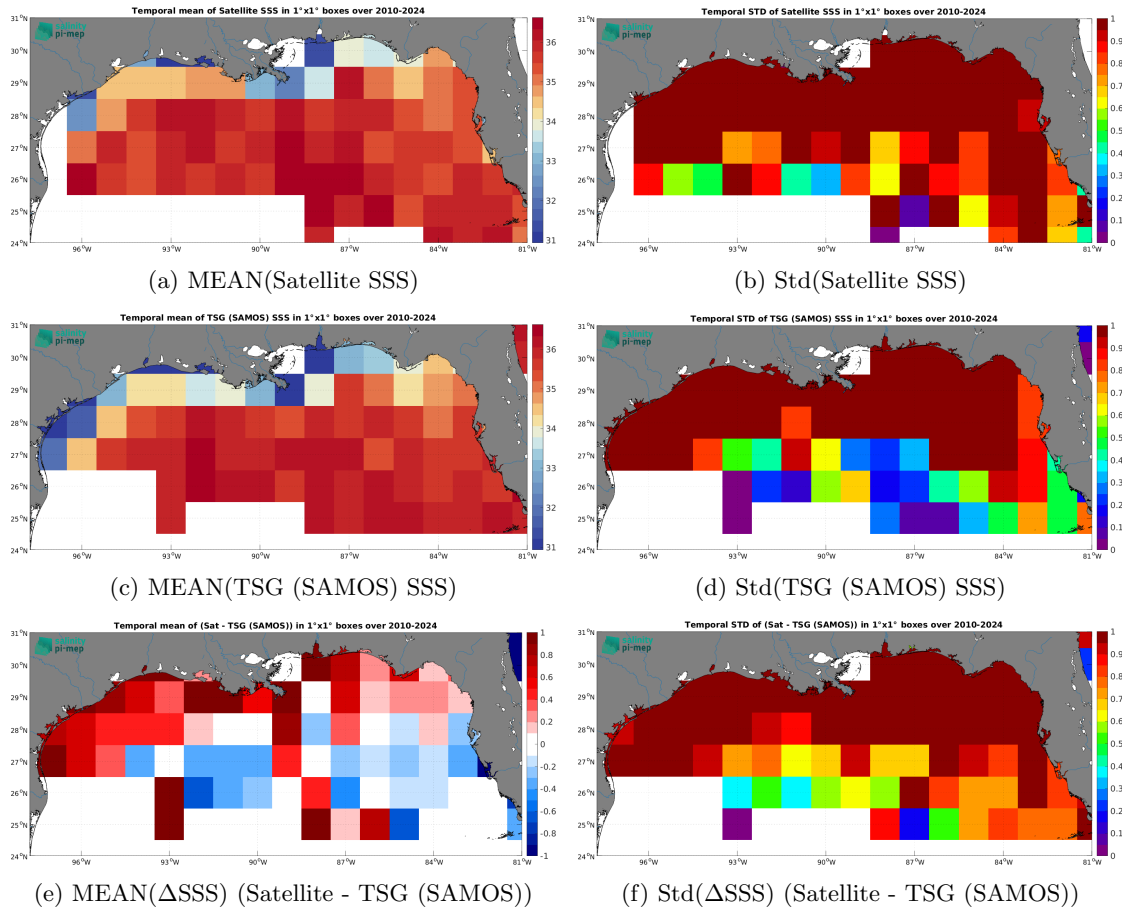
Figure 7: Temporal mean (left) and Std (right) of SSS from SMOS SSS L2 v700 (ESA) (top), TSG (SAMOS) (middle), and of \Delta SSS (Satellite - TSG (SAMOS)). Only match-up pairs are used to generate these maps.
