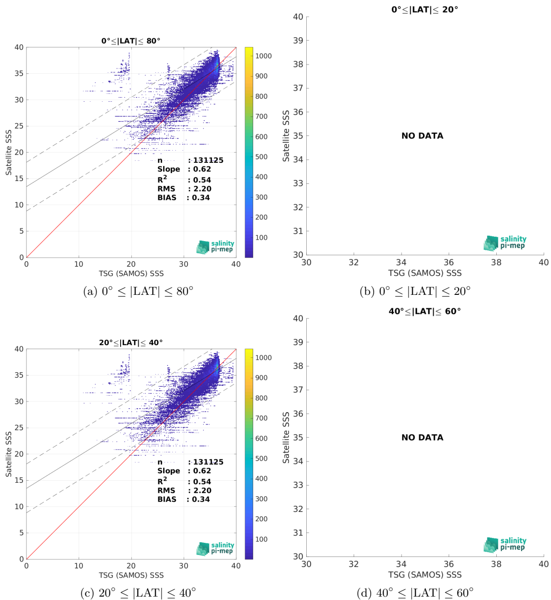
Figure 10: Contour maps of the concentration of SMOS SSS L2 v700 (ESA) SSS (y-axis) versus TSG (SAMOS) SSS (x-axis) at match-up pairs for different latitude bands. For each plot, the red line shows x=y . The black thin and dashed lines indicate a linear fit through the data cloud and the \pm 95\% confidence levels, respectively. The number match-up pairs n , the slope and R^2 coefficient of the linear fit, the root mean square (RMS) and the mean bias between satellite and in situ data are indicated for each latitude band in each plots.
