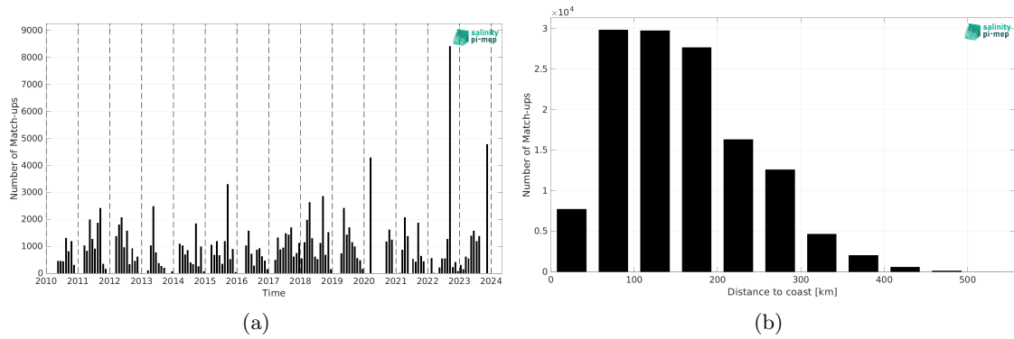
Figure 2: Number of match-ups between TSG (SAMOS) and SMOS SSS L2 v700 (ESA) SSS as a function of time (a) and as function of the distance to coast (b) over the Mississippi river plume Pi-MEP region and for the full satellite product period.
