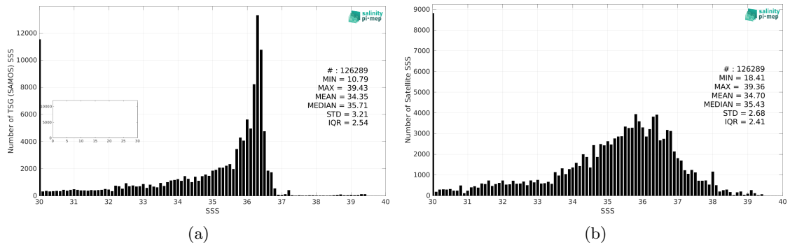
Figure 2: Histograms of SSS from TSG (SAMOS) (a) and SMOS SSS L2 v700 (ESA) (b) considering all match-up pairs per bins of 0.1 over the Mississippi river plume Pi-MEP region and for the full satellite product period.
