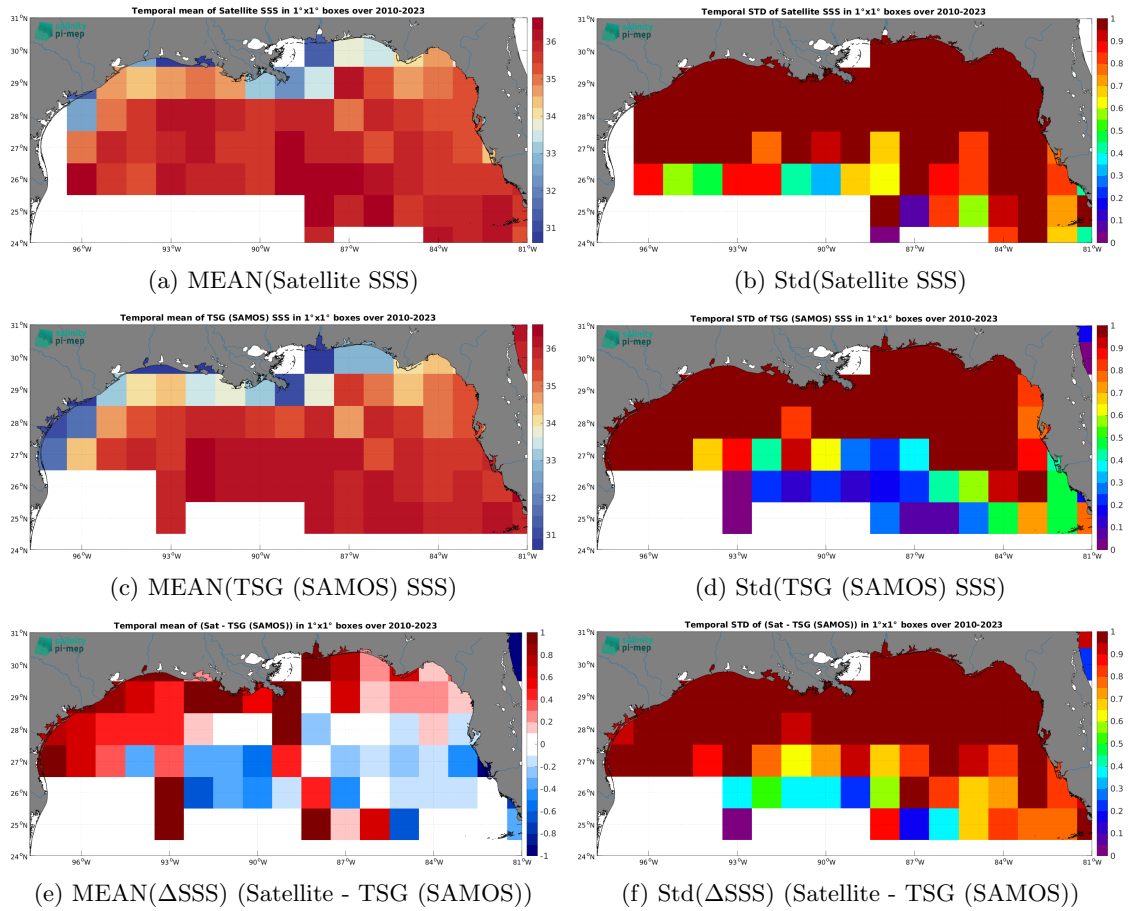
Figure 6: Temporal mean (left) and Std (right) of SSS from SMOS SSS L2 v700 (ESA) (top), TSG (SAMOS) (middle), and of \Delta SSS (Satellite - TSG (SAMOS)). Only match-up pairs are used to generate these maps.
