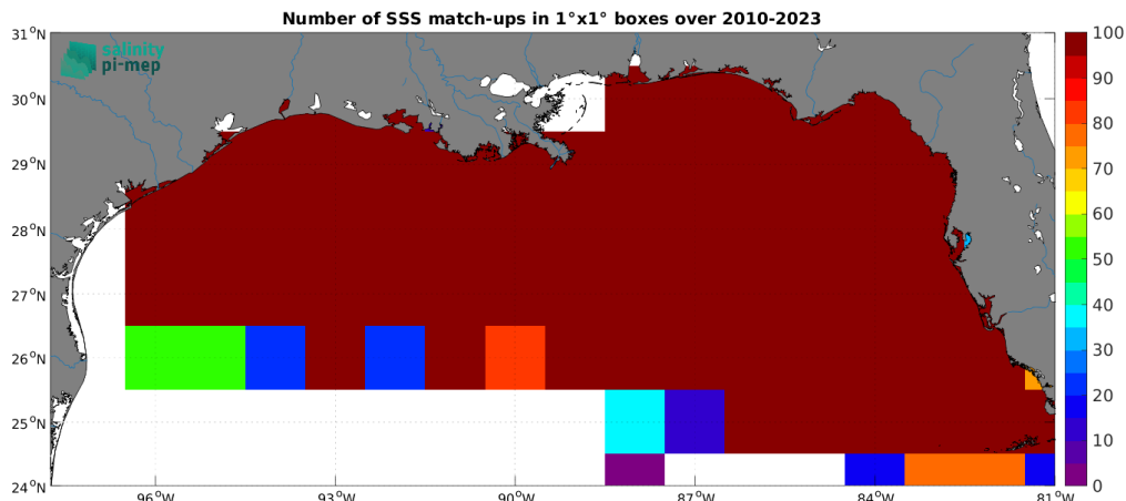
Figure 4: Number of SSS match-ups between TSG (SAMOS) SSS and the SMOS SSS L2 v700 (ESA) SSS product for the Mississippi river plume Pi-MEP region over 1^\circ \times 1^\circ boxes and for the full satellite product period.
