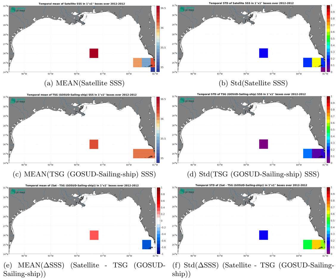
Figure 6: Temporal mean (left) and Std (right) of SSS from SMOS SSS L2 v700 (ESA) (top), TSG (GOSUD-Sailing-ship) (middle), and of \Delta SSS (Satellite - TSG (GOSUD-Sailing-ship)). Only match-up pairs are used to generate these maps.
