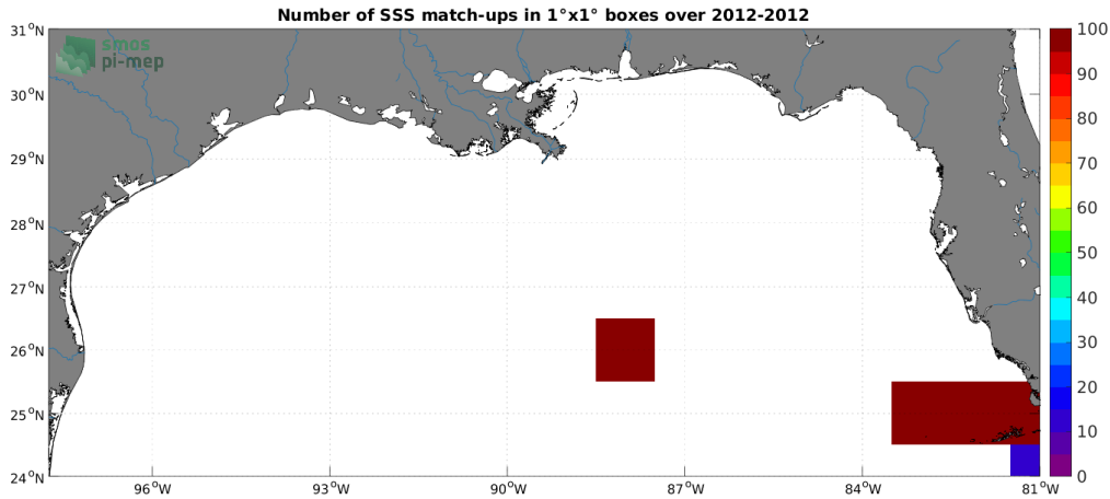
Figure 4: Number of SSS match-ups between TSG (GOSUD-Sailing-ship) SSS and the SMOS SSS L2 v700 (ESA) SSS product for the Mississippi river plume Pi-MEP region over 1^\circ \times 1^\circ boxes and for the full satellite product period.
