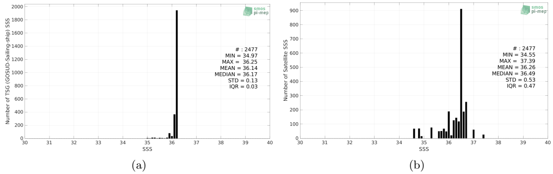
Figure 2: Histograms of SSS from TSG (GOSUD-Sailing-ship) (a) and SMOS SSS L2 v700 (ESA) (b) considering all match-up pairs per bins of 0.1 over the Mississippi river plume Pi-MEP region and for the full satellite product period.
