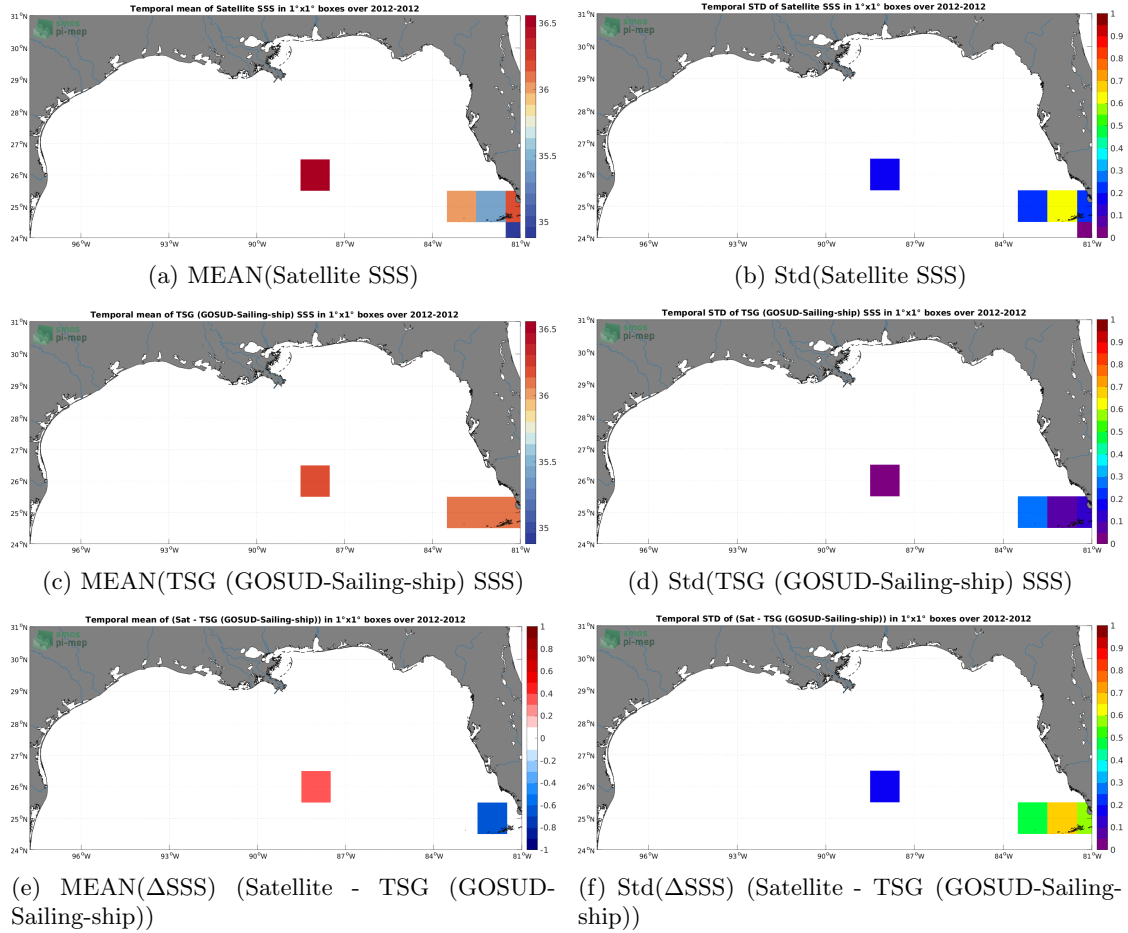
Figure 6: Temporal mean (left) and Std (right) of SSS from SMOS SSS L2 v700 (ESA) (top), TSG (GOSUD-Sailing-ship) (middle), and of \Delta\text{SSS} (Satellite - TSG (GOSUD-Sailing-ship)). Only match-up pairs are used to generate these maps.
