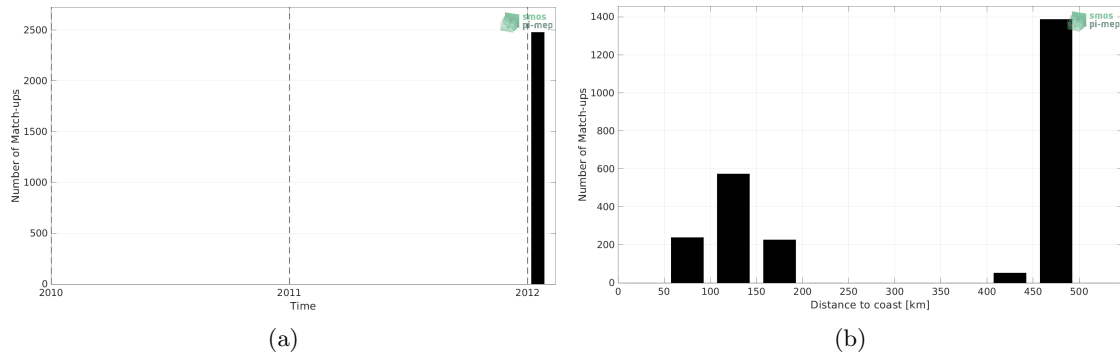
Figure 1: Number of match-ups between TSG (GOSUD-Sailing-ship) and SMOS SSS L2 v700 (ESA) SSS as a function of time (a) and as function of the distance to coast (b) over the Mississippi river plume Pi-MEP region and for the full satellite product period.
