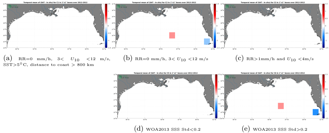
Figure 12: Temporal mean gridded over spatial boxes of size 1^{\circ}\times 1^{\circ} of \Delta SSS (SMOS SSS L2 v700 (ESA) - TSG (GOSUD-Sailing-ship)) for 5 different subdatasets corresponding to:RR=0 mm/h, 3 < U_{10} < 12 m/s, SST >5^{\circ}\text{C} , distance to coast > 800 km (a), RR=0 mm/h, 3 < U_{10} < 12 m/s (b), RR >1 mm/h and U_{10} < 4 m/s (c), WOA2013 SSS Std <0.2 (d), WOA2013 SSS Std >0.2 (e).
