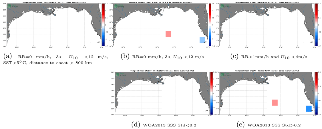
Figure 12: Temporal mean gridded over spatial boxes of size 1^\circ \times 1^\circ of \Delta SSS (SMOS SSS L2 v700 (ESA) - TSG (GOSUD-Sailing-ship)) for 5 different subdatasets corresponding to: RR=0 mm/h, 3 < U_{10} < 12 m/s, SST > 5^\circ\text{C} , distance to coast > 800 km (a), RR=0 mm/h, 3 < U_{10} < 12 m/s (b), RR > 1 mm/h and U_{10} < 4 m/s (c), WOA2013 SSS Std < 0.2 (d), WOA2013 SSS Std > 0.2 (e).
