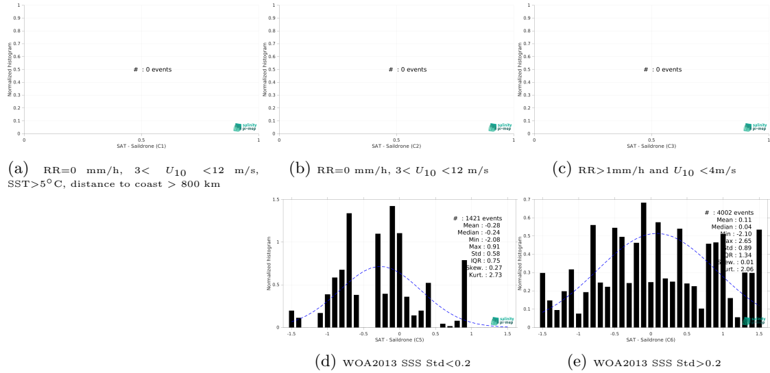
Figure 15: Normalized histogram of \Delta\text{SSS} (SMOS SSS L2 v700 (ESA) - Saiclone) for 5 different subdatasets corresponding to: RR=0 mm/h, 3 < U_{10} < 12 m/s, SST>5°C, distance to coast > 800 km (a), RR=0 mm/h, 3 < U_{10} < 12 m/s (b), RR>1mm/h and U_{10} < 4 m/s (c), WOA2013 SSS Std<0.2 (d), WOA2013 SSS Std>0.2 (e).
