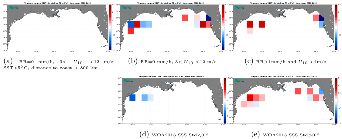
Figure 12: Temporal mean gridded over spatial boxes of size 1^{\circ}\times 1^{\circ} of \Delta\text{SSS} (SMOS SSS L2 v700 (ESA) - Saifdrone) for 5 different subdatasets corresponding to:RR=0 mm/h, 3 < U_{10} < 12 m/s, SST >5^{\circ}\text{C} , distance to coast > 800 km (a), RR=0 mm/h, 3 < U_{10} < 12 m/s (b), RR >1 mm/h and U_{10} < 4 m/s (c), WOA2013 SSS Std <0.2 (d), WOA2013 SSS Std >0.2 (e).
