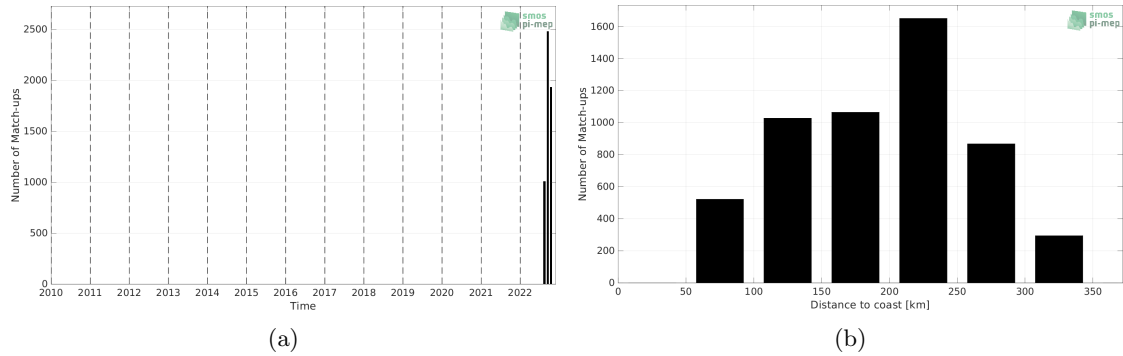
Figure 1: Number of match-ups between Saildrone and SMOS SSS L2 v700 (ESA) SSS as a function of time (a) and as function of the distance to coast (b) over the Mississippi river plume Pi-MEP region and for the full satellite product period.
