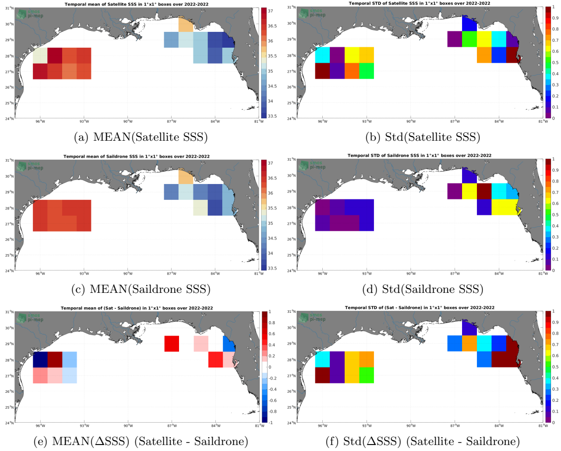
Figure 6: Temporal mean (left) and Std (right) of SSS from SMOS SSS L2 v700 (ESA) (top), Saildrone (middle), and of \Delta SSS (Satellite - Saildrone). Only match-up pairs are used to generate these maps.
