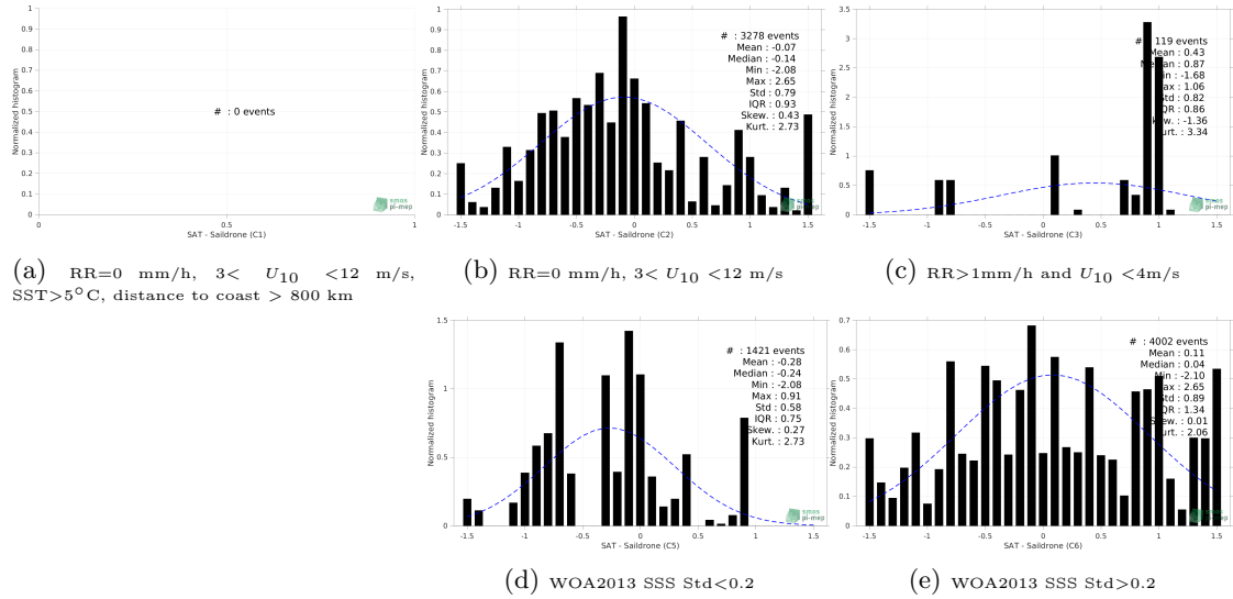
Figure 13: Normalized histogram of \Delta SSS (SMOS SSS L2 v700 (ESA) - Sairdrone) for 5 different subdatasets corresponding to: RR=0 mm/h, 3 < U_{10} < 12 m/s, SST > 5°C, distance to coast > 800 km (a), RR=0 mm/h, 3 < U_{10} < 12 m/s (b), RR > 1mm/h and U_{10} < 4 m/s (c), WOA2013 SSS Std < 0.2 (d), WOA2013 SSS Std > 0.2 (e).
