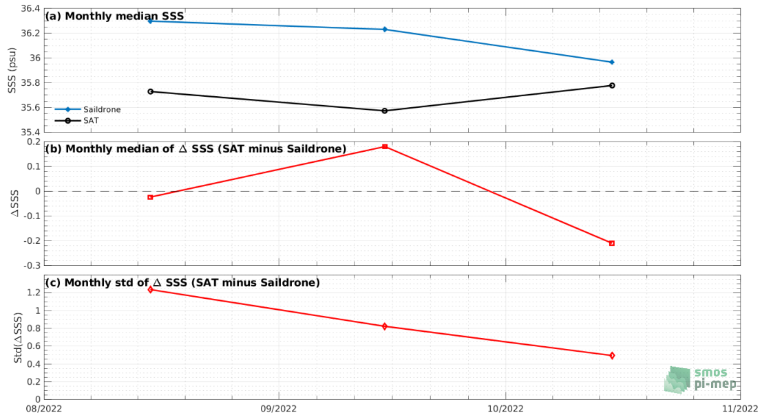
Figure 7: Time series of the monthly median SSS (top), median of \Delta SSS (Satellite - Sairdrone) and Std of \Delta SSS (Satellite - Sairdrone) over the Mississippi river plume Pi-MEP region considering all match-ups collected by the Pi-MEP.
