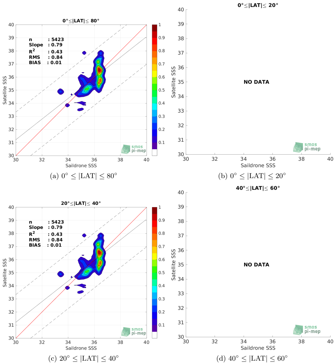
Figure 9: Contour maps of the concentration of SMOS SSS L2 v700 (ESA) SSS (y-axis) versus Saïldrone SSS (x-axis) at match-up pairs for different latitude bands. For each plot, the red line shows x=y . The black thin and dashed lines indicate a linear fit through the data cloud and the \pm 95\% confidence levels, respectively. The number match-up pairs n , the slope and R^2 coefficient of the linear fit, the root mean square (RMS) and the mean bias between satellite and in situ data are indicated for each latitude band in each plots.
