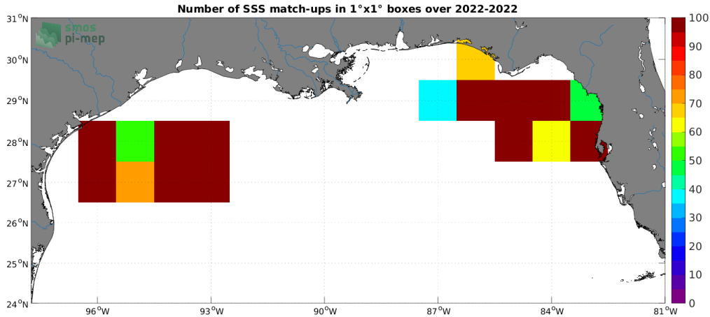
Figure 4: Number of SSS match-ups between Saildrone SSS and the SMOS SSS L2 v700 (ESA) SSS product for the Mississippi river plume Pi-MEP region over 1^\circ \times 1^\circ boxes and for the full satellite product period.
