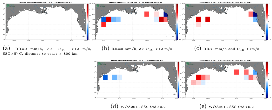
Figure 12: Temporal mean gridded over spatial boxes of size 1^{\circ}\times 1^{\circ} of \Delta\text{SSS} (SMOS SSS L2 v700 (ESA) - Sairdrone) for 5 different subdatasets corresponding to:RR=0 mm/h, 3 < U_{10} < 12 m/s, SST >5^{\circ}\text{C} , distance to coast > 800 km (a), RR=0 mm/h, 3 < U_{10} < 12 m/s (b), RR >1 mm/h and U_{10} < 4 m/s (c), WOA2013 SSS Std <0.2 (d), WOA2013 SSS Std >0.2 (e).
