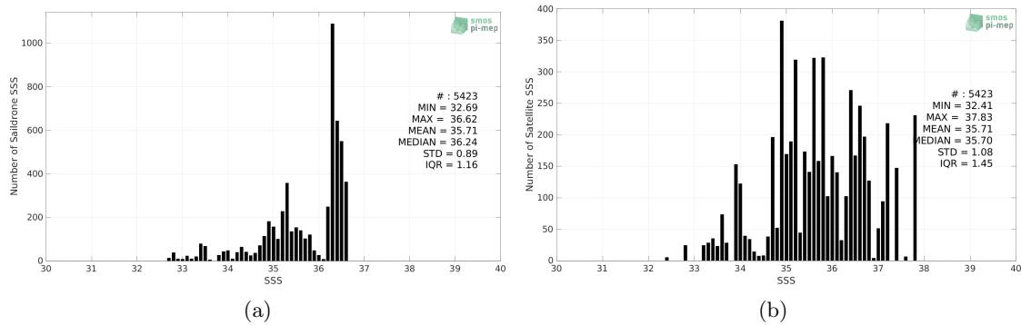
Figure 2: Histograms of SSS from Saildrone (a) and SMOS SSS L2 v700 (ESA) (b) considering all match-up pairs per bins of 0.1 over the Mississippi river plume Pi-MEP region and for the full satellite product period.
