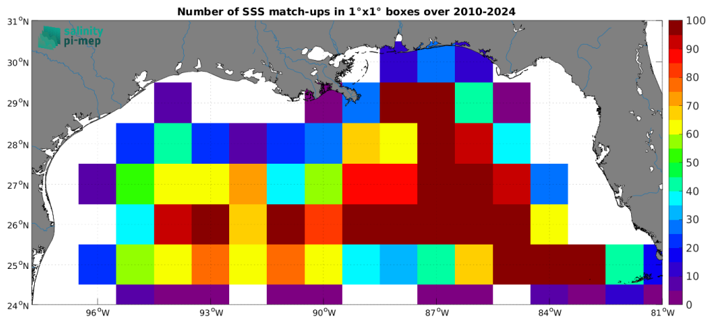
Figure 5: Number of SSS match-ups between Argo SSS and the SMOS SSS L2 v700 (ESA) SSS product for the Mississippi river plume Pi-MEP region over 1^\circ \times 1^\circ boxes and for the full satellite product period.
