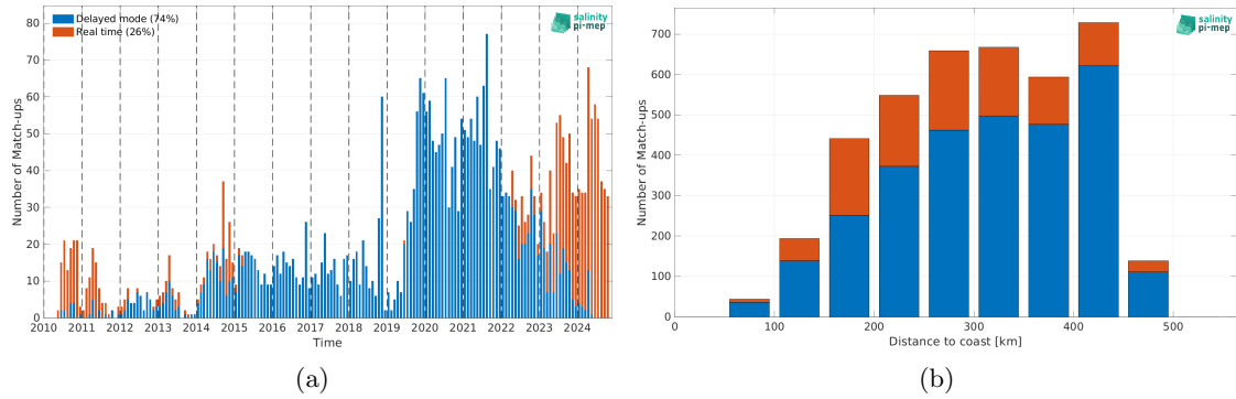
Figure 2: Number of match-ups between Argo and SMOS SSS L2 v700 (ESA) SSS as a function of time (a) and as function of the distance to coast (b) over the Mississippi river plume Pi-MEP region and for the full satellite product period.
