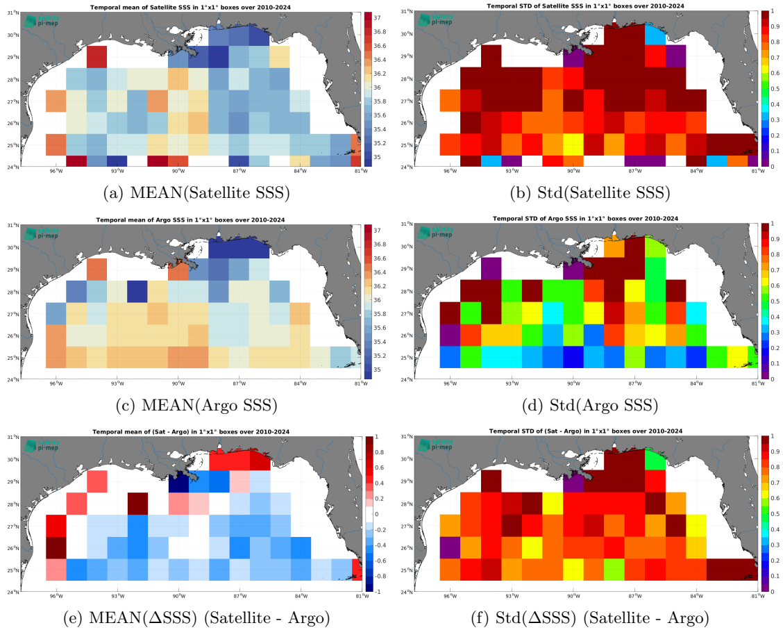
Figure 7: Temporal mean (left) and Std (right) of SSS from SMOS SSS L2 v700 (ESA) (top), Argo (middle), and of \Delta SSS (Satellite - Argo). Only match-up pairs are used to generate these maps.
