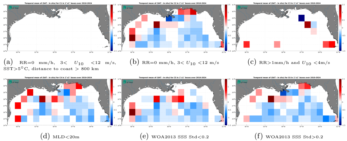
Figure 14: Temporal mean gridded over spatial boxes of size 1^\circ \times 1^\circ of \Delta SSS (SMOS SSS L2 v700 (ESA) - Argo) for 6 different subdatasets corresponding to:RR=0 mm/h, 3 < U_{10} < 12 m/s, SST>5°C, distance to coast > 800 km (a), RR=0 mm/h, 3 < U_{10} < 12 m/s (b), RR>1mm/h and U_{10} < 4 m/s (c),MLD<20m (d),WOA2013 SSS Std<0.2 (e),WOA2013 SSS Std>0.2 (f).
