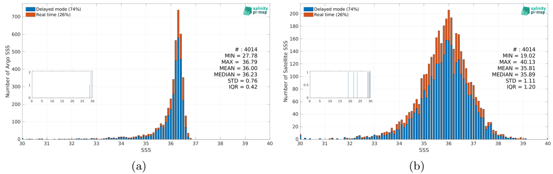
Figure 3: Histograms of SSS from Argo (a) and SMOS SSS L2 v700 (ESA) (b) considering all match-up pairs per bins of 0.1 over the Mississippi river plume Pi-MEP region and for the full satellite product period.
