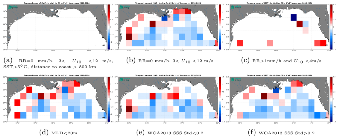
Figure 14: Temporal mean gridded over spatial boxes of size 1^\circ \times 1^\circ of \Delta SSS (SMOS SSS L2 v700 (ESA) - Argo) for 6 different subdatasets corresponding to: RR=0 mm/h, 3 < U_{10} < 12 m/s, SST > 5^\circ\text{C} , distance to coast > 800 km (a), RR=0 mm/h, 3 < U_{10} < 12 m/s (b), RR > 1 mm/h and U_{10} < 4 m/s (c), MLD < 20 m (d), WOA2013 SSS Std < 0.2 (e), WOA2013 SSS Std > 0.2 (f).
