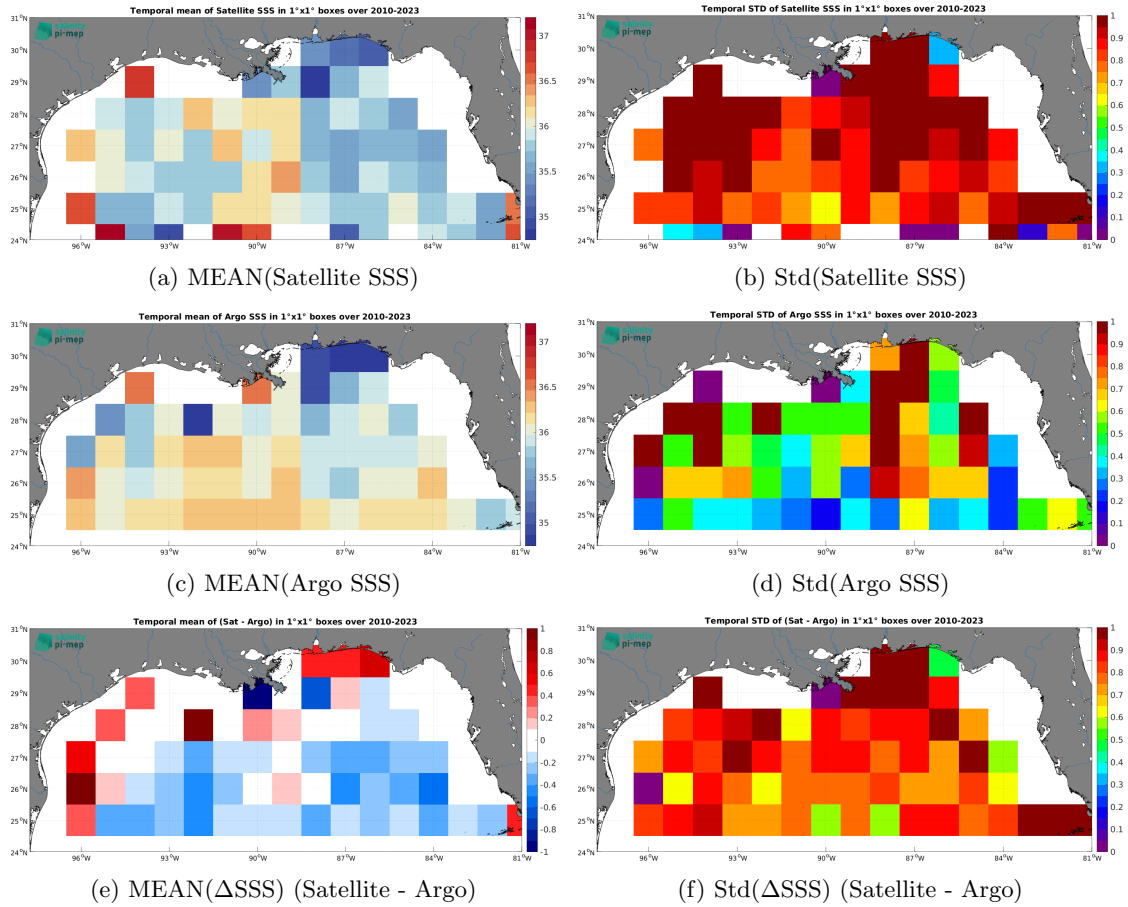
Figure 6: Temporal mean (left) and Std (right) of SSS from SMOS SSS L2 v700 (ESA) (top), Argo (middle), and of \Delta SSS (Satellite - Argo). Only match-up pairs are used to generate these maps.
