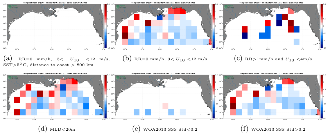
Figure 12: Temporal mean gridded over spatial boxes of size 1^{\circ}\times 1^{\circ} of \Delta\text{SSS} (SMOS SSS L2 v700 (ESA) - Argo) for 6 different subdatasets corresponding to:RR=0 mm/h, 3 < U_{10} < 12 m/s, SST >5^{\circ}\text{C} , distance to coast > 800 km (a), RR=0 mm/h, 3 < U_{10} < 12 m/s (b), RR >1 mm/h and U_{10} < 4\text{m/s} (c),MLD <20\text{m} (d),WOA2013 SSS Std <0.2 (e),WOA2013 SSS Std >0.2 (f).
