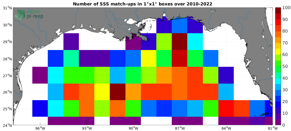
Figure 4: Number of SSS match-ups between Argo SSS and the SMOS SSS L2 v700 (ESA) SSS product for the Mississippi river plume Pi-MEP region over 1^\circ \times 1^\circ boxes and for the full satellite product period.
