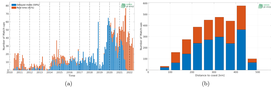
Figure 1: Number of match-ups between Argo and SMOS SSS L2 v700 (ESA) SSS as a function of time (a) and as function of the distance to coast (b) over the Mississippi river plume Pi-MEP region and for the full satellite product period.
