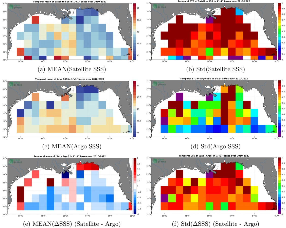
Figure 6: Temporal mean (left) and Std (right) of SSS from SMOS SSS L2 v700 (ESA) (top), Argo (middle), and of \Delta\text{SSS} (Satellite - Argo). Only match-up pairs are used to generate these maps.
