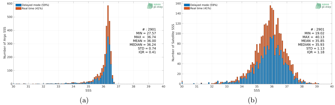
Figure 2: Histograms of SSS from Argo (a) and SMOS SSS L2 v700 (ESA) (b) considering all match-up pairs per bins of 0.1 over the Mississippi river plume Pi-MEP region and for the full satellite product period.
