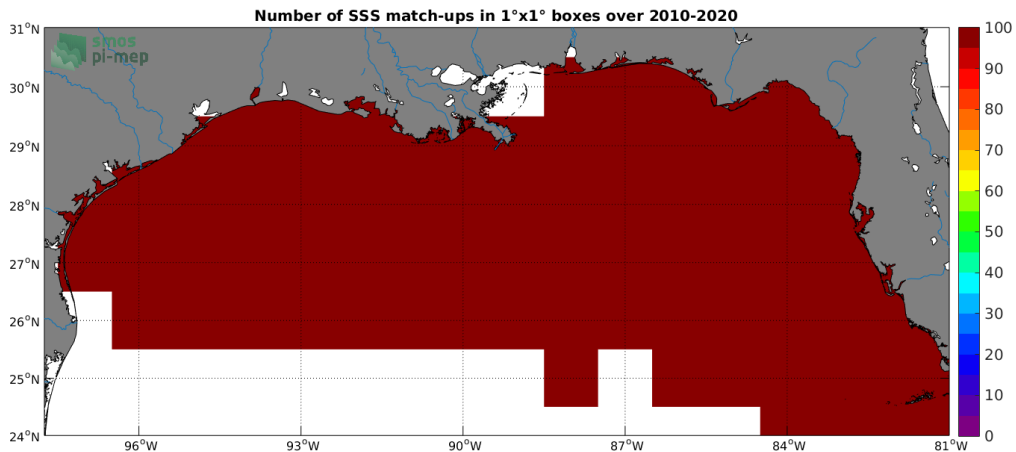
Figure 4: Number of SSS match-ups between TSG (SAMOS) SSS and the SMOS SSS L2 v662 (ESA) SSS product for the Mississippi river plume Pi-MEP region over 1°x1° boxes and for the full satellite product period.
