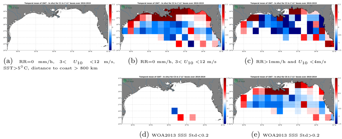
Figure 12: Temporal mean gridded over spatial boxes of size 1^{\circ}\times 1^{\circ} of \Delta\text{SSS} (SMOS L2 v662 (ESA) - TSG-SAMOS) for 5 different subdatasets corresponding to:RR=0 mm/h, 3 < U_{10} < 12 m/s, SST > 5^{\circ}\text{C} , distance to coast > 800 km (a), RR=0 mm/h, 3 < U_{10} < 12 m/s (b), RR > 1 mm/h and U_{10} < 4 m/s (c), WOA2013 SSS Std < 0.2 (d), WOA2013 SSS Std > 0.2 (e).
