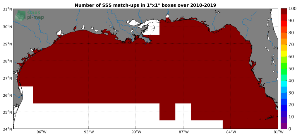
Figure 4: Number of SSS match-ups between TSG-SAMOS SSS and the SMOS L2 v662 (ESA) SSS product for the Mississippi river plume Pi-MEP region over 1^\circ \times 1^\circ boxes and for the full satellite product period.
