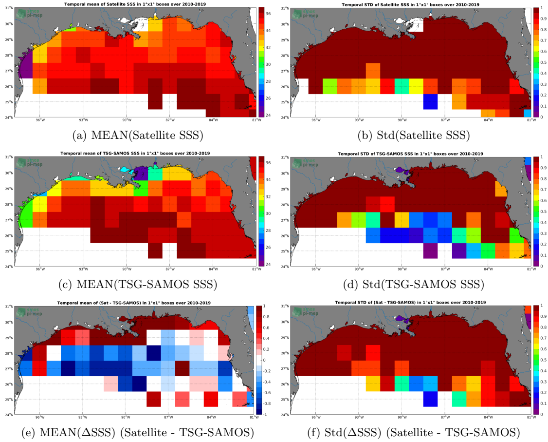
Figure 6: Temporal mean (left) and Std (right) of SSS from SMOS L2 v662 (ESA) (top), TSG-SAMOS (middle), and of \Delta SSS (Satellite - TSG-SAMOS). Only match-up pairs are used to generate these maps.
