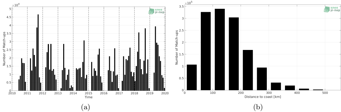
Figure 1: Number of match-ups between TSG-SAMOS and SMOS L2 v662 (ESA) SSS as a function of time (a) and as function of the distance to coast (b) over the Mississippi river plume Pi-MEP region and for the full satellite product period.
