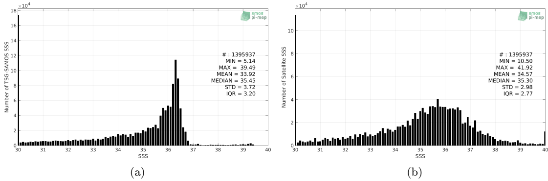
Figure 2: Histograms of SSS from TSG-SAMOS (a) and SMOS L2 v662 (ESA) (b) considering all match-up pairs per bins of 0.1 over the Mississippi river plume Pi-MEP region and for the full satellite product period.
