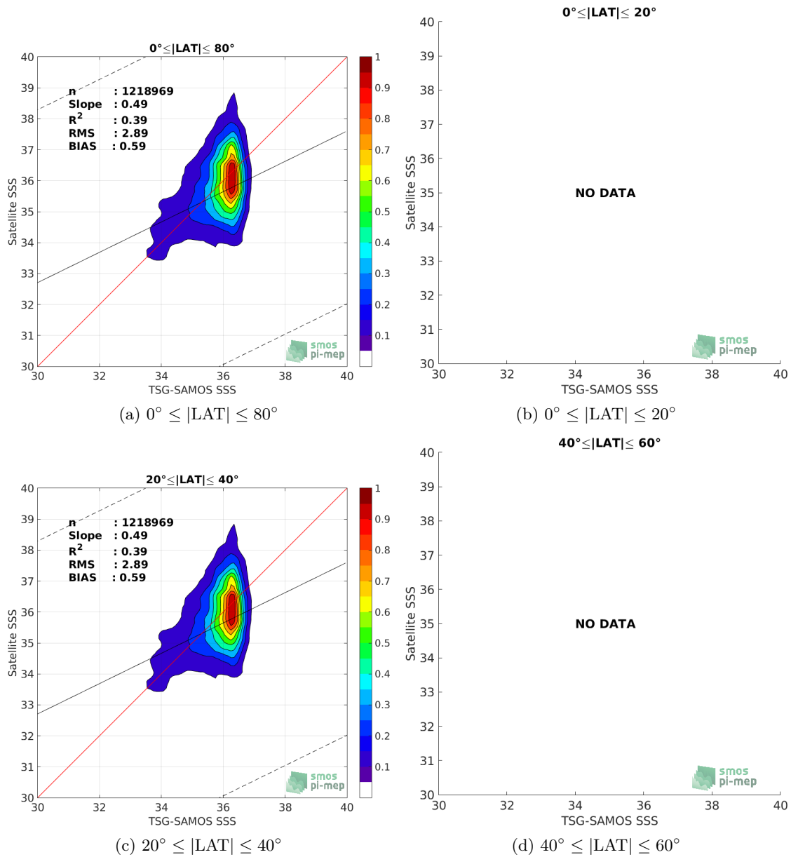
Figure 9: Contour maps of the concentration of SMOS-L2-DPGS-v662 SSS ( y -axis) versus TSG-SAMOS SSS ( x -axis) at match-up pairs for different latitude bands. For each plot, the red line shows x=y . The black thin and dashed lines indicate a linear fit through the data cloud and the \pm 95\% confidence levels, respectively. The number match-up pairs n , the slope and R^2 coefficient of the linear fit, the root mean square (RMS) and the mean bias between satellite and in situ data are indicated for each latitude band in each plots.
