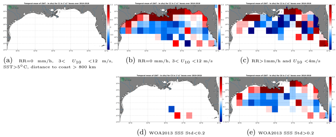
Figure 12: Temporal mean gridded over spatial boxes of size 1^\circ \times 1^\circ of \Delta SSS (SMOS-L2-DPGS-v662 - TSG-SAMOS) for 5 different subdatasets corresponding to: RR=0 mm/h, 3 < U_{10} < 12 m/s, SST > 5^\circ C , distance to coast > 800 km (a), RR=0 mm/h, 3 < U_{10} < 12 m/s (b), RR > 1 mm/h and U_{10} < 4 m/s (c), WOA2013 SSS Std < 0.2 (d), WOA2013 SSS Std > 0.2 (e).
