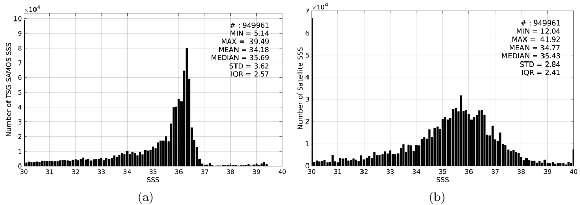
Figure 2: Histograms of SSS from TSG-SAMOS (a) and SMOS-L2-DPGS-v662 (b) considering all match-up pairs per bins of 0.1 over the Mississippi river plume Pi-MEP region and for the full satellite product period.
