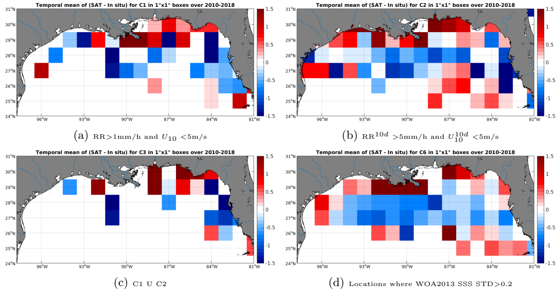
Figure 12: Temporal mean gridded over spatial boxes of size 1^\circ \times 1^\circ of \Delta SSS (SMOS-L2-DPGS-v662 - TSG-SAMOS) for 4 different subdatasets corresponding to:RR >1 mm/h and U_{10} < 5 m/s (a), RR 10d > 5 mm/h and U_{10}^{10d} < 5 m/s (b), C1 U C2 (c),Locations where WOA2013 SSS STD >0.2 (d).
