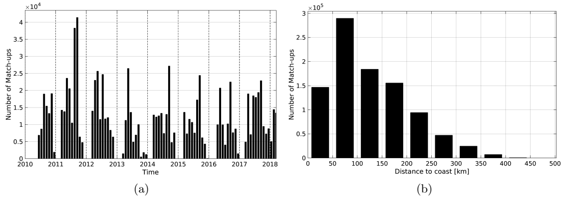
Figure 1: Number of match-ups between TSG-SAMOS and SMOS-L2-DPGS-v662 SSS as a function of time (a) and as function of the distance to coast (b) over the Mississippi river plume Pi-MEP region and for the full satellite product period.
