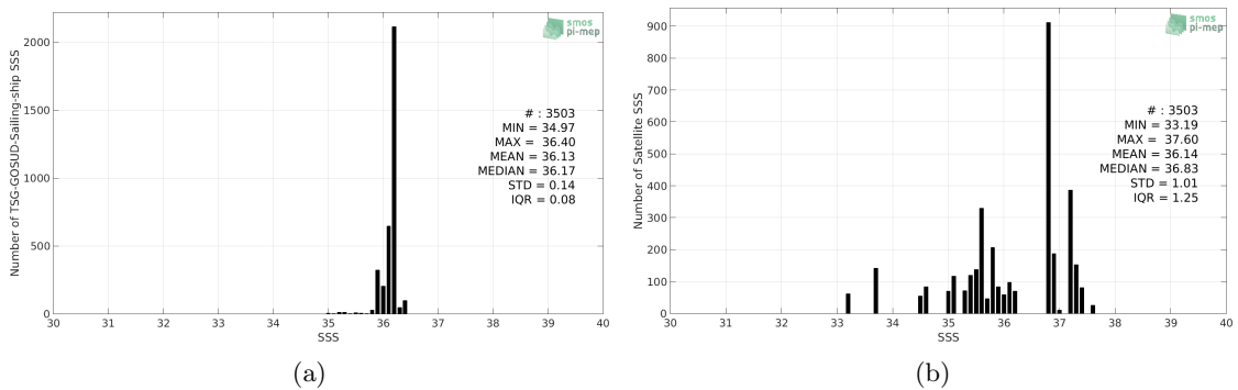
Figure 2: Histograms of SSS from TSG-GOSUD-Sailing-ship (a) and SMOS L2 v662 (ESA) (b) considering all match-up pairs per bins of 0.1 over the Mississippi river plume Pi-MEP region and for the full satellite product period.
