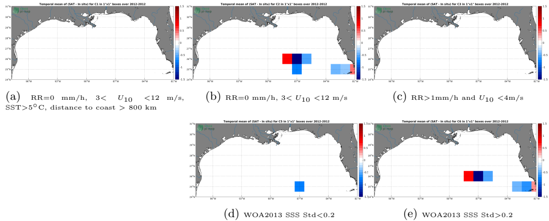
Figure 12: Temporal mean gridded over spatial boxes of size 1^{\circ}\times 1^{\circ} of \Delta SSS (SMOS L2 v662 (ESA) - TSG-GOSUD-Sailing-ship) for 5 different subdatasets corresponding to:RR=0 mm/h, 3 < U_{10} < 12 m/s, SST >5^{\circ}\text{C} , distance to coast > 800 km (a), RR=0 mm/h, 3 < U_{10} < 12 m/s (b), RR >1 mm/h and U_{10} < 4 m/s (c), WOA2013 SSS Std <0.2 (d), WOA2013 SSS Std >0.2 (e).
