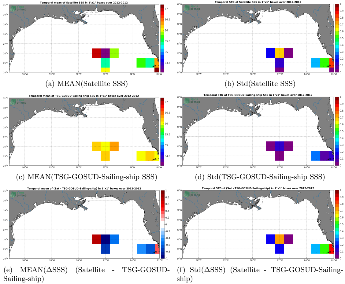
Figure 6: Temporal mean (left) and Std (right) of SSS from SMOS L2 v662 (ESA) (top), TSG-GOSUD-Sailing-ship (middle), and of \Delta SSS (Satellite - TSG-GOSUD-Sailing-ship). Only match-up pairs are used to generate these maps.
