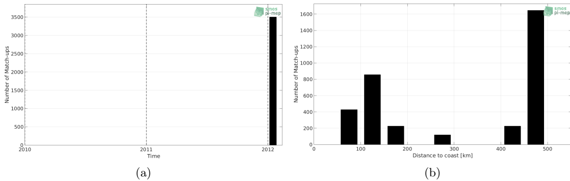
Figure 1: Number of match-ups between TSG-GOSUD-Sailing-ship and SMOS L2 v662 (ESA) SSS as a function of time (a) and as function of the distance to coast (b) over the Mississippi river plume Pi-MEP region and for the full satellite product period.
