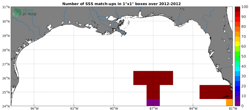
Figure 4: Number of SSS match-ups between TSG-GOSUD-Sailing-ship SSS and the SMOS L2 v662 (ESA) SSS product for the Mississippi river plume Pi-MEP region over 1^\circ \times 1^\circ boxes and for the full satellite product period.
