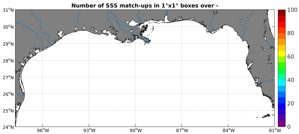
Figure 4: Number of SSS match-ups between TSG-GOSUD-Research-vessel SSS and the SMOS-L2-DPGS-v662 SSS product for the Mississippi river plume Pi-MEP region over 1^\circ \times 1^\circ boxes and for the full satellite product period.
