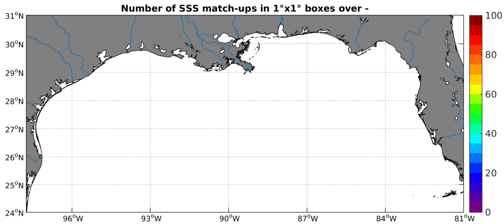
Figure 3: Number of SSS match-ups between Surface drifters SSS and the SMOS-L2-DPGS-v662 SSS product for the Mississippi river plume Pi-MEP region over 1^\circ \times 1^\circ boxes and for the full satellite product period.
