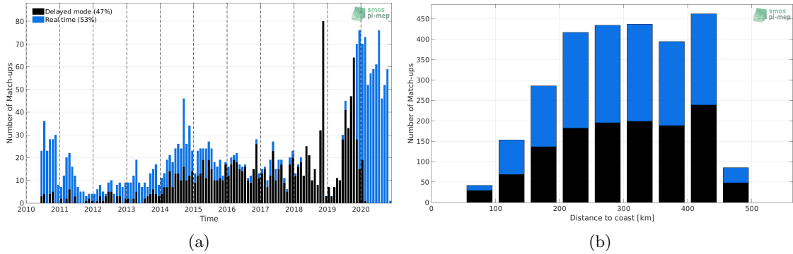
Figure 1: Number of match-ups between Argo and SMOS SSS L2 v662 (ESA) SSS as a function of time (a) and as function of the distance to coast (b) over the Mississippi river plume Pi-MEP region and for the full satellite product period.
