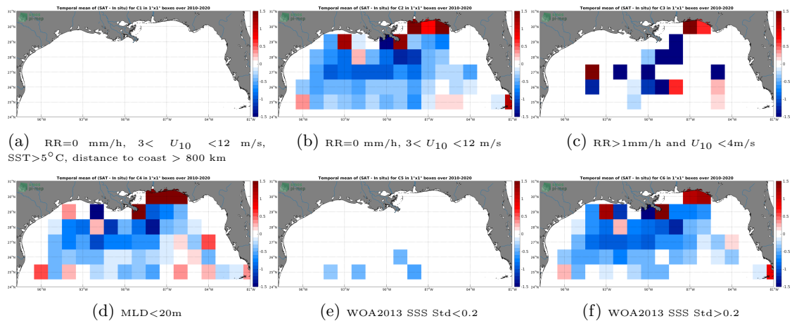
Figure 12: Temporal mean gridded over spatial boxes of size 1^{\circ}\times 1^{\circ} of \Delta\text{SSS} (SMOS SSS L2 v662 (ESA) - Argo) for 6 different subdatasets corresponding to:RR=0 mm/h, 3 < U_{10} < 12 m/s, SST > 5^{\circ}\text{C} , distance to coast > 800 km (a), RR=0 mm/h, 3 < U_{10} < 12 m/s (b), RR > 1\text{mm/h} and U_{10} < 4\text{m/s} (c),MLD < 20\text{m} (d),WOA2013 SSS Std < 0.2 (e),WOA2013 SSS Std > 0.2 (f).
