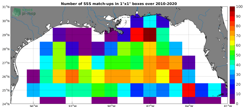
Figure 4: Number of SSS match-ups between Argo SSS and the SMOS SSS L2 v662 (ESA) SSS product for the Mississippi river plume Pi-MEP region over 1°x1° boxes and for the full satellite product period.
