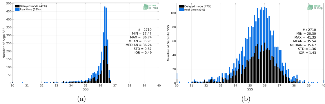
Figure 2: Histograms of SSS from Argo (a) and SMOS SSS L2 v662 (ESA) (b) considering all match-up pairs per bins of 0.1 over the Mississippi river plume Pi-MEP region and for the full satellite product period.
