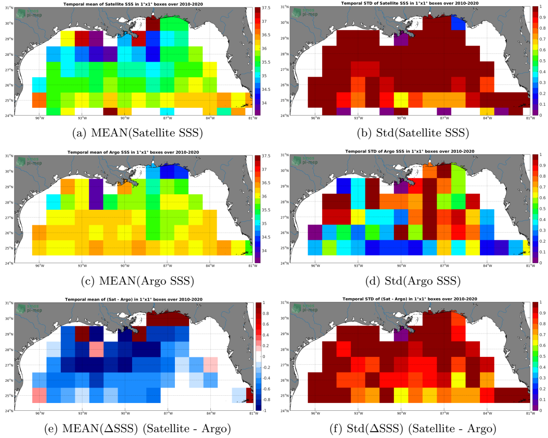
Figure 6: Temporal mean (left) and Std (right) of SSS from SMOS SSS L2 v662 (ESA) (top), Argo (middle), and of \Delta SSS (Satellite - Argo). Only match-up pairs are used to generate these maps.
