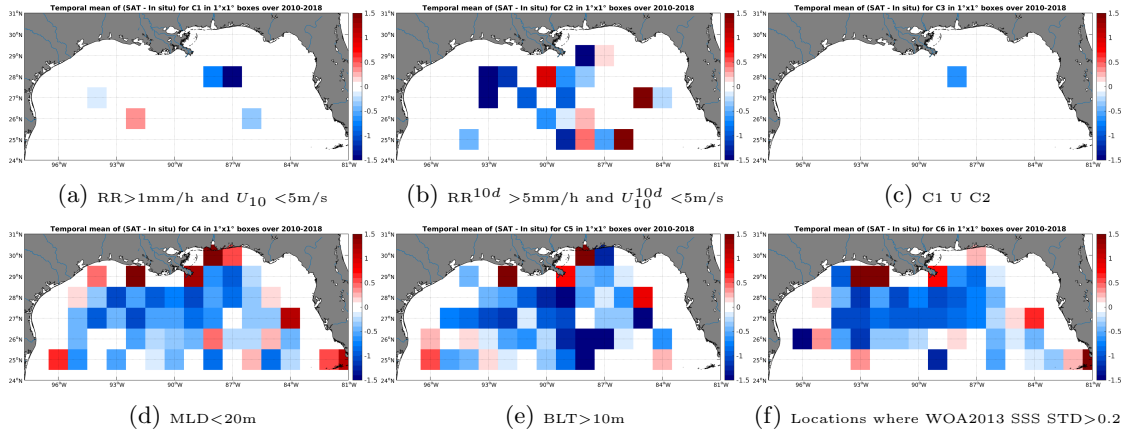
Figure 12: Temporal mean gridded over spatial boxes of size 1^\circ \times 1^\circ of \Delta\text{SSS} (SMOS-L2-DPGS-v662 - Argo) for 6 different subdatasets corresponding to: \text{RR} > 1\text{mm/h} and U_{10} < 5\text{m/s} (a), \text{RR}^{10d} > 5\text{mm/h} and U_{10}^{10d} < 5\text{m/s} (b), C1 U C2 (c), \text{MLD} < 20\text{m} (d), \text{BLT} > 10\text{m} (e), Locations where WOA2013 SSS STD > 0.2 (f).
