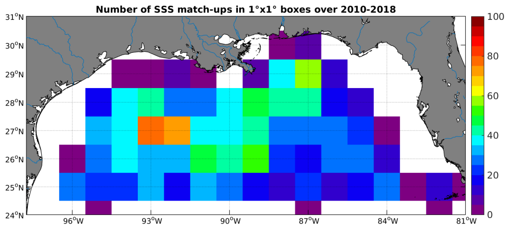
Figure 4: Number of SSS match-ups between Argo SSS and the SMOS-L2-DPGS-v662 SSS product for the Mississippi river plume Pi-MEP region over 1^\circ \times 1^\circ boxes and for the full satellite product period.
