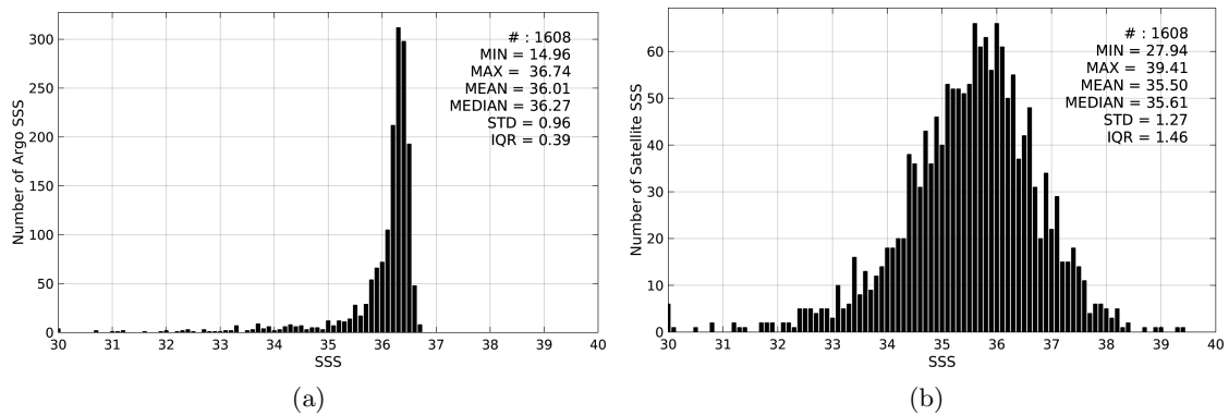
Figure 2: Histograms of SSS from Argo (a) and SMOS-L2-DPGS-v662 (b) considering all match-up pairs per bins of 0.1 over the Mississippi river plume Pi-MEP region and for the full satellite product period.
