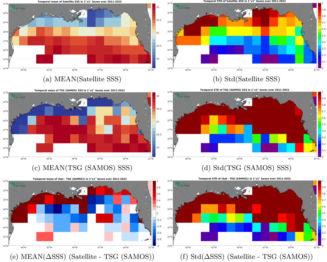
Figure 6: Temporal mean (left) and Std (right) of SSS from SMAP SSS L4 OI v1 - 7 Days (IPRC) (top), TSG (SAMOS) (middle), and of \Delta\text{SSS} (Satellite - TSG (SAMOS)). Only match-up pairs are used to generate these maps.
