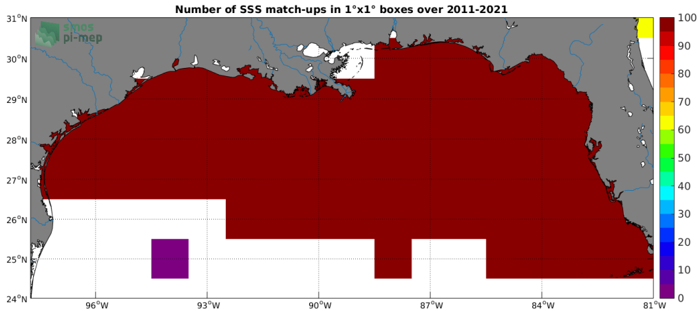
Figure 4: Number of SSS match-ups between TSG (SAMOS) SSS and the SMAP SSS L4 OI v1 - 7day (IPRC) SSS product for the Mississippi river plume Pi-MEP region over 1^\circ \times 1^\circ boxes and for the full satellite product period.
