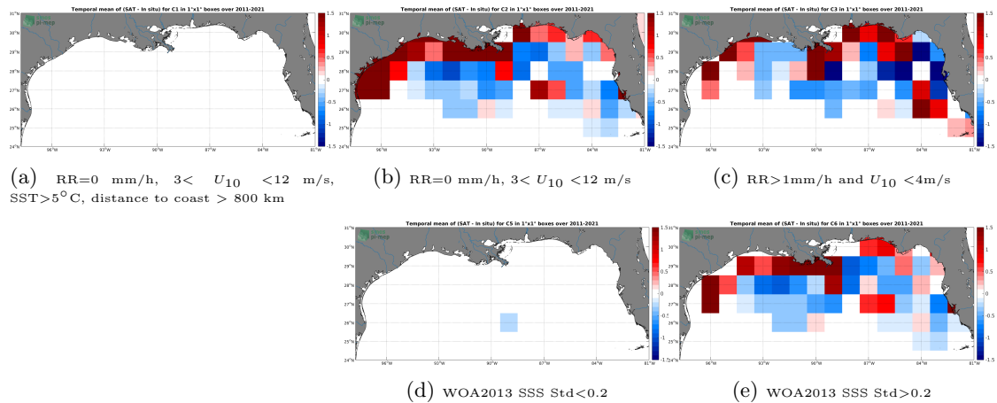
Figure 12: Temporal mean gridded over spatial boxes of size 1^{\circ}\times 1^{\circ} of \Delta\text{SSS} (SMAP SSS L4 OI v1 - 7day (IPRC) - TSG (SAMOS)) for 5 different subdatasets corresponding to:RR=0 mm/h, 3 < U_{10} < 12 m/s, SST >5^{\circ}\text{C} , distance to coast > 800 km (a), RR=0 mm/h, 3 < U_{10} < 12 m/s (b), RR >1 mm/h and U_{10} < 4 m/s (c), WOA2013 SSS Std <0.2 (d), WOA2013 SSS Std >0.2 (e).
