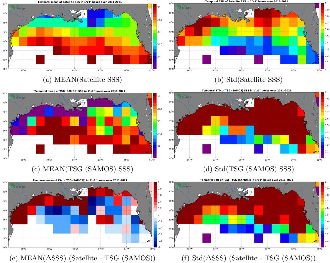
Figure 6: Temporal mean (left) and Std (right) of SSS from SMAP SSS L4 OI v1 - 7day (IPRC) (top), TSG (SAMOS) (middle), and of \Delta\text{SSS} (Satellite - TSG (SAMOS)). Only match-up pairs are used to generate these maps.
