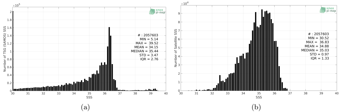
Figure 2: Histograms of SSS from TSG (SAMOS) (a) and SMAP SSS L4 OI v1 - 7day (IPRC) (b) considering all match-up pairs per bins of 0.1 over the Mississippi river plume Pi-MEP region and for the full satellite product period.
