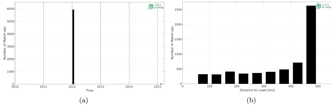
Figure 1: Number of match-ups between TSG (GOSUD-Sailing-ship) and SMAP SSS L4 OI v1 - 7day (IPRC) SSS as a function of time (a) and as function of the distance to coast (b) over the Mississippi river plume Pi-MEP region and for the full satellite product period.
