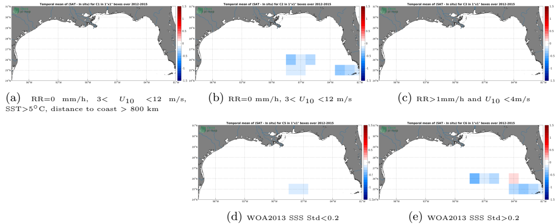
Figure 12: Temporal mean gridded over spatial boxes of size 1^{\circ}\times 1^{\circ} of \Delta SSS (SMAP SSS L4 OI v1 - 7day (IPRC) - TSG (GOSUD-Sailing-ship)) for 5 different subdatasets corresponding to: RR=0 mm/h, 3 < U_{10} < 12 m/s, SST > 5^{\circ}\text{C} , distance to coast > 800 km (a), RR=0 mm/h, 3 < U_{10} < 12 m/s (b), RR > 1 mm/h and U_{10} < 4 m/s (c), WOA2013 SSS Std < 0.2 (d), WOA2013 SSS Std > 0.2 (e).
