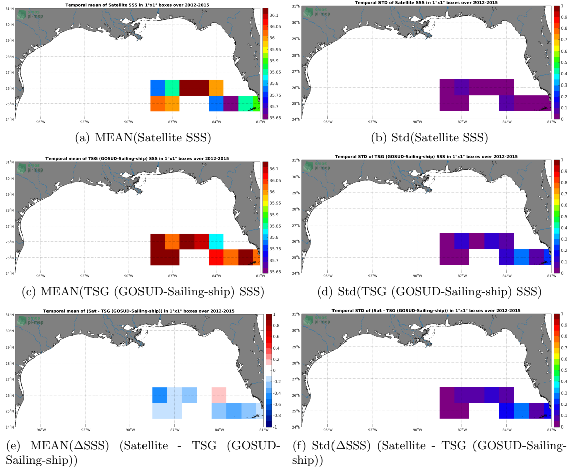
Figure 6: Temporal mean (left) and Std (right) of SSS from SMAP SSS L4 OI v1 - 7day (IPRC) (top), TSG (GOSUD-Sailing-ship) (middle), and of \Delta SSS (Satellite - TSG (GOSUD-Sailing-ship)). Only match-up pairs are used to generate these maps.
