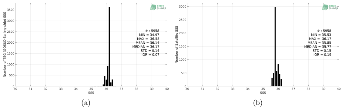
Figure 2: Histograms of SSS from TSG (GOSUD-Sailing-ship) (a) and SMAP SSS L4 OI v1 - 7day (IPRC) (b) considering all match-up pairs per bins of 0.1 over the Mississippi river plume Pi-MEP region and for the full satellite product period.
