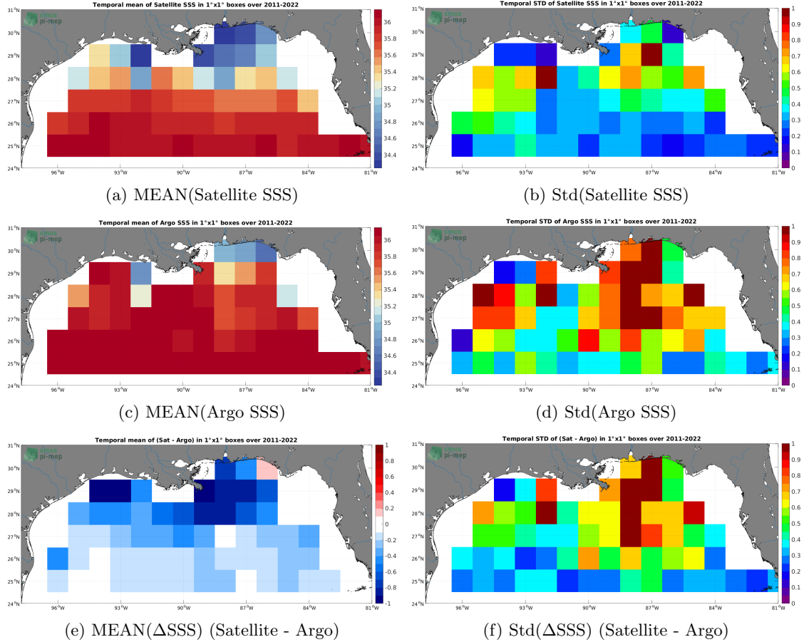
Figure 6: Temporal mean (left) and Std (right) of SSS from SMAP SSS L4 OI v1 - 7 Days (IPRC) (top), Argo (middle), and of \Delta\text{SSS} (Satellite - Argo). Only match-up pairs are used to generate these maps.
