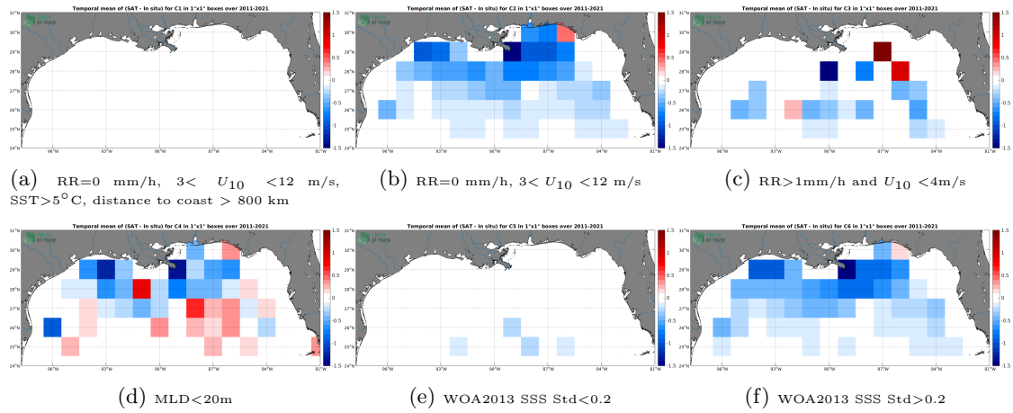
Figure 12: Temporal mean gridded over spatial boxes of size 1^{\circ}\times 1^{\circ} of \Delta\text{SSS} (SMAP SSS L4 OI v1 - 7 Days (IPRC) - Argo) for 6 different subdatasets corresponding to:RR=0 mm/h, 3 < U_{10} < 12 m/s, SST >5^{\circ}\text{C} , distance to coast > 800 km (a), RR=0 mm/h, 3 < U_{10} < 12 m/s (b), RR >1\text{mm/h} and U_{10} < 4\text{m/s} (c),MLD <20\text{m} (d),WOA2013 SSS Std <0.2 (e),WOA2013 SSS Std >0.2 (f).
