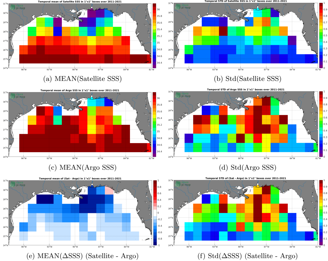
Figure 6: Temporal mean (left) and Std (right) of SSS from SMAP SSS L4 OI v1 - 7day (IPRC) (top), Argo (middle), and of \Delta\text{SSS} (Satellite - Argo). Only match-up pairs are used to generate these maps.
