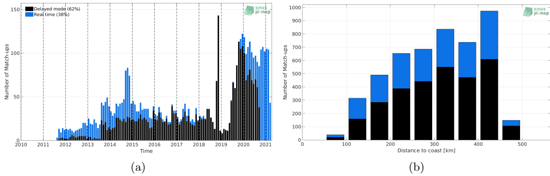
Figure 1: Number of match-ups between Argo and SMAP SSS L4 OI v1 - 7day (IPRC) SSS as a function of time (a) and as function of the distance to coast (b) over the Mississippi river plume Pi-MEP region and for the full satellite product period.
