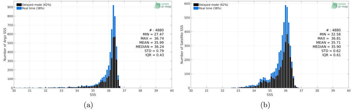
Figure 2: Histograms of SSS from Argo (a) and SMAP SSS L4 OI v1 - 7day (IPRC) (b) considering all match-up pairs per bins of 0.1 over the Mississippi river plume Pi-MEP region and for the full satellite product period.
