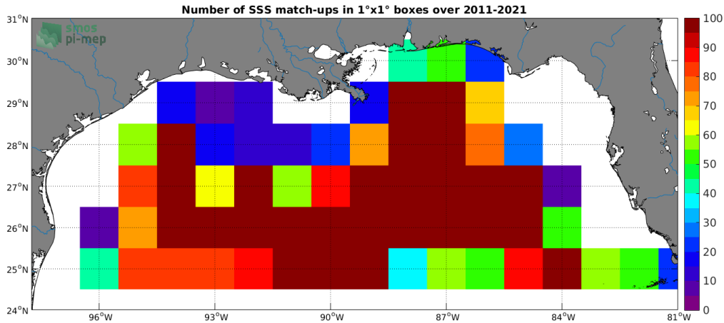
Figure 4: Number of SSS match-ups between Argo SSS and the SMAP SSS L4 OI v1 - 7day (IPRC) SSS product for the Mississippi river plume Pi-MEP region over 1°x1° boxes and for the full satellite product period.
