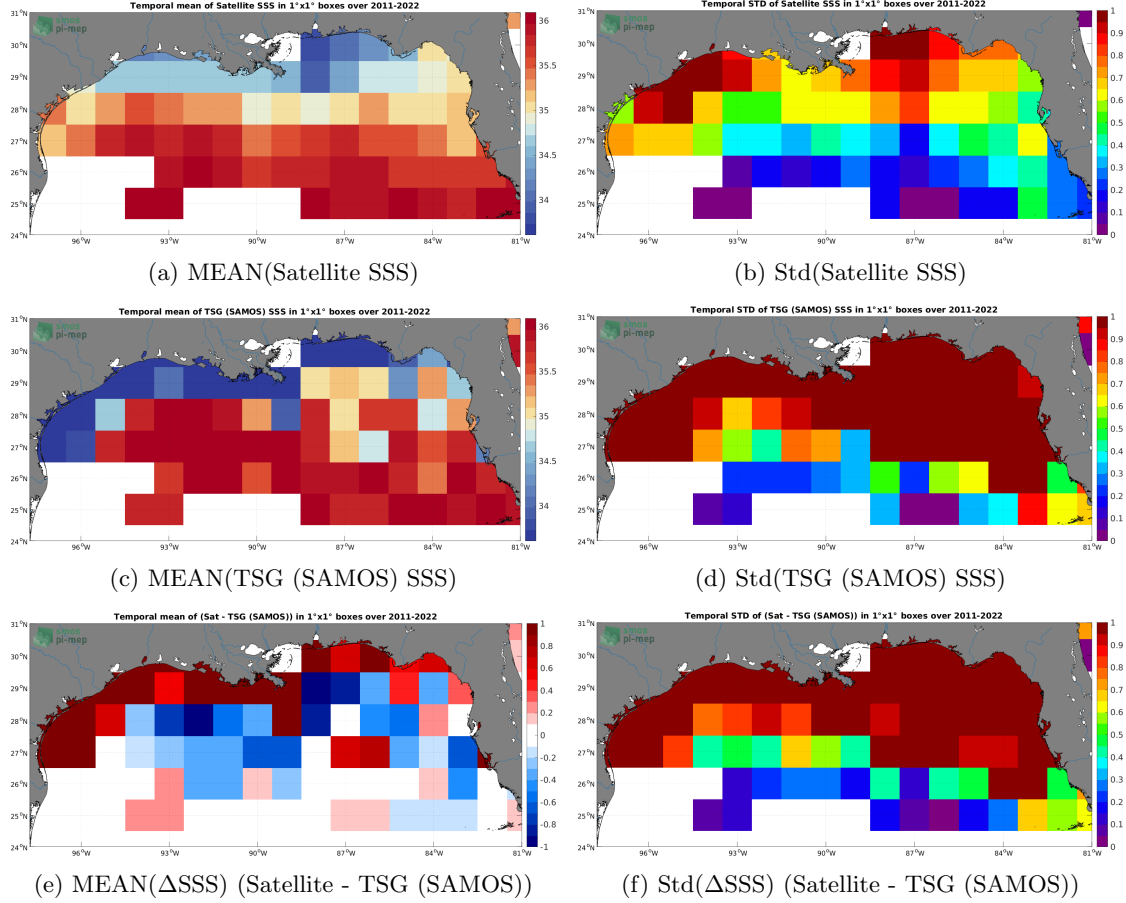
Figure 6: Temporal mean (left) and Std (right) of SSS from SMAP SSS L4 OI v1 - Monthly (IPRC) (top), TSG (SAMOS) (middle), and of \Delta\text{SSS} (Satellite - TSG (SAMOS)). Only match-up pairs are used to generate these maps.
