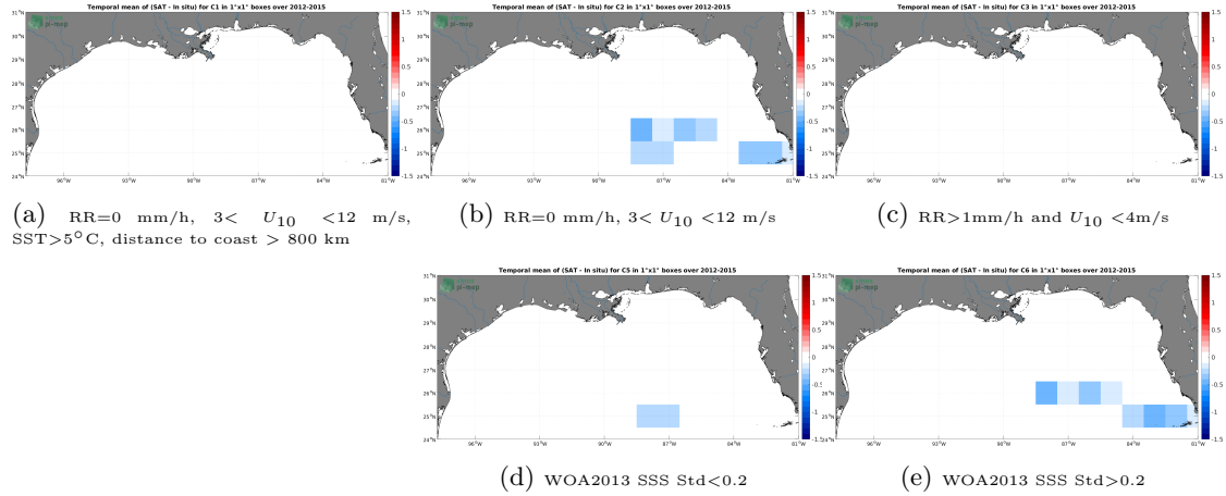
Figure 12: Temporal mean gridded over spatial boxes of size 1^{\circ}\times 1^{\circ} of \Delta SSS (SMAP SSS L4 OI v1 - Monthly (IPRC) - TSG (GOSUD-Sailing-ship)) for 5 different subdatasets corresponding to:RR=0 mm/h, 3 < U_{10} < 12 m/s, SST >5^{\circ}\text{C} , distance to coast > 800 km (a), RR=0 mm/h, 3 < U_{10} < 12 m/s (b), RR >1 mm/h and U_{10} < 4 m/s (c), WOA2013 SSS Std <0.2 (d), WOA2013 SSS Std >0.2 (e).
