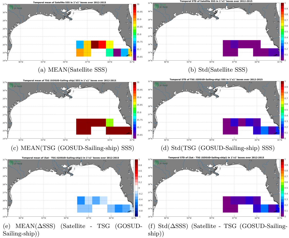
Figure 6: Temporal mean (left) and Std (right) of SSS from SMAP SSS L4 OI v1 - Monthly (IPRC) (top), TSG (GOSUD-Sailing-ship) (middle), and of \Delta SSS (Satellite - TSG (GOSUD-Sailing-ship)). Only match-up pairs are used to generate these maps.
