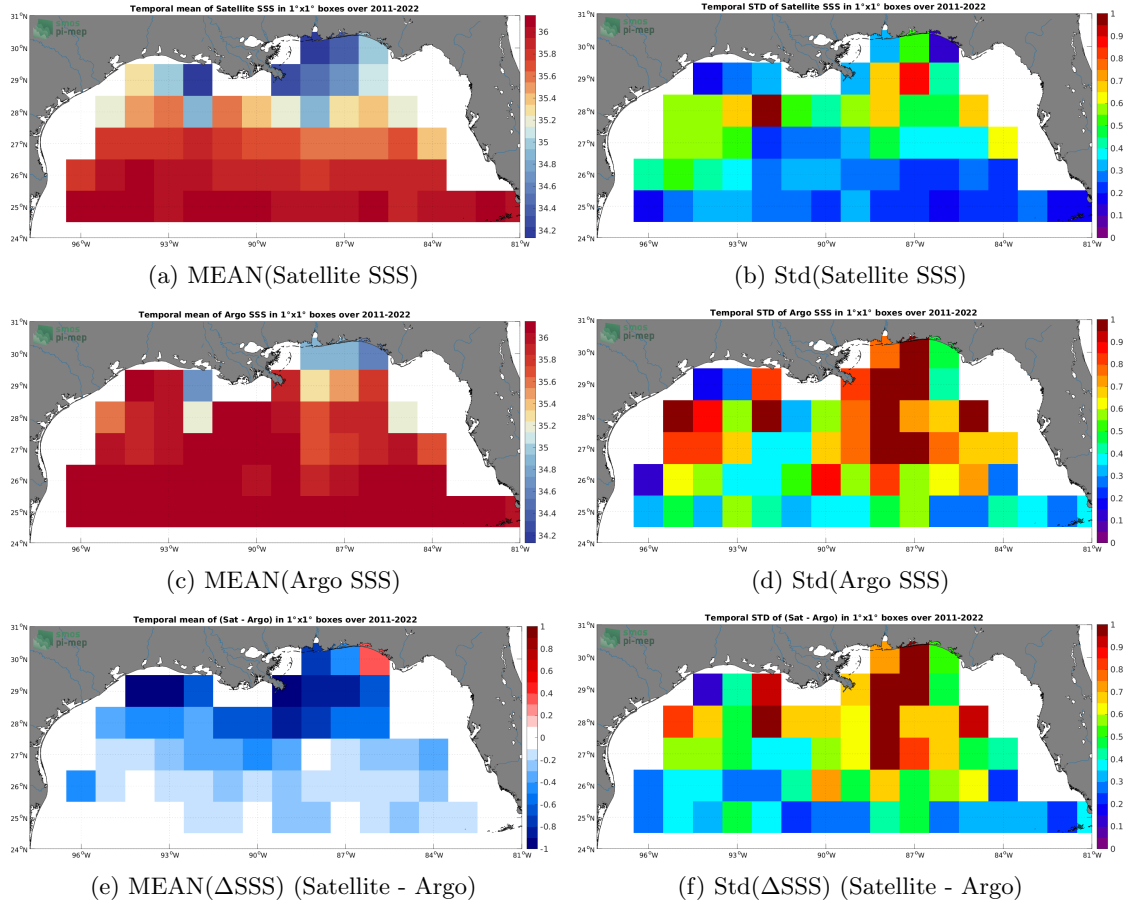
Figure 6: Temporal mean (left) and Std (right) of SSS from SMAP SSS L4 OI v1 - Monthly (IPRC) (top), Argo (middle), and of \Delta\text{SSS} (Satellite - Argo). Only match-up pairs are used to generate these maps.
