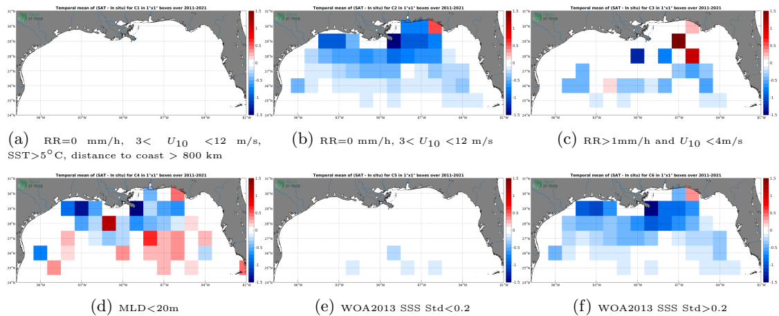
Figure 12: Temporal mean gridded over spatial boxes of size 1^{\circ}\times 1^{\circ} of \Delta\text{SSS} (SMAP SSS L4 OI v1 - Monthly (IPRC) - Argo) for 6 different subdatasets corresponding to:RR=0 mm/h, 3 < U_{10} < 12 m/s, SST > 5^{\circ}\text{C} , distance to coast > 800 km (a), RR=0 mm/h, 3 < U_{10} < 12 m/s (b), RR > 1\text{mm/h} and U_{10} < 4\text{m/s} (c),MLD < 20\text{m} (d),WOA2013 SSS Std < 0.2 (e),WOA2013 SSS Std > 0.2 (f).
