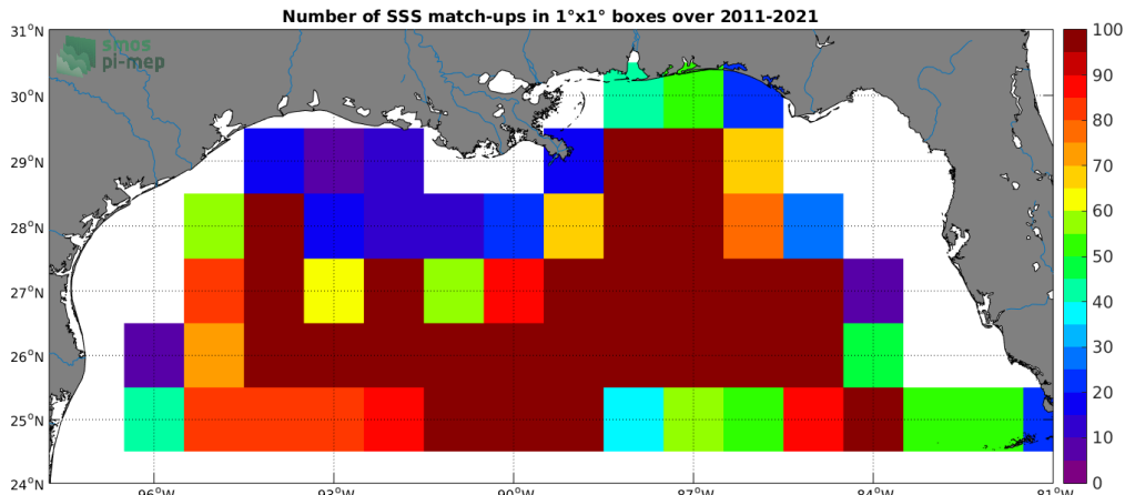
Figure 4: Number of SSS match-ups between Argo SSS and the SMAP SSS L4 OI v1 - Monthly (IPRC) SSS product for the Mississippi river plume Pi-MEP region over 1°x1° boxes and for the full satellite product period.
