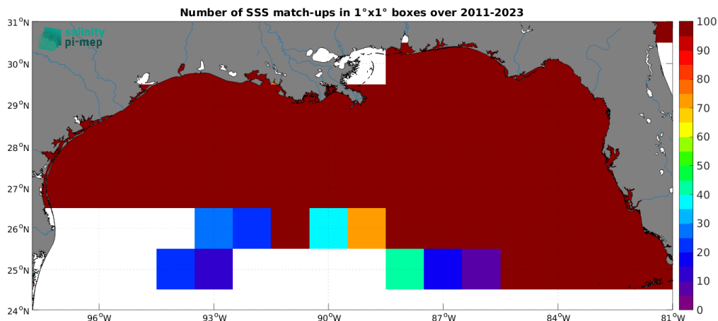
Figure 5: Number of SSS match-ups between TSG (SAMOS) SSS and the SMAP SSS L4 OI v3 - Monthly (ESR) SSS product for the Mississippi river plume Pi-MEP region over 1^\circ \times 1^\circ boxes and for the full satellite product period.
