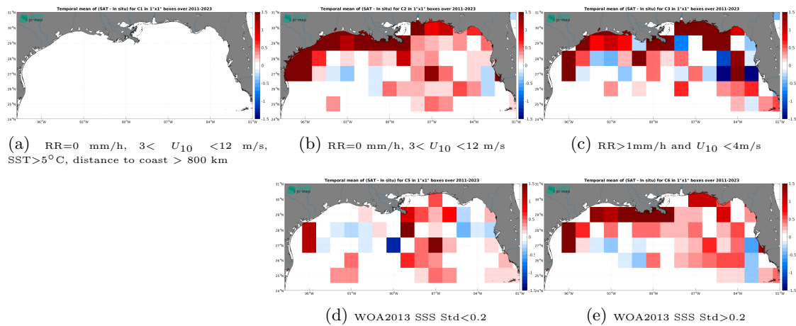
Figure 14: Temporal mean gridded over spatial boxes of size 1^\circ \times 1^\circ of \Delta SSS (SMAP SSS L4 OI v3 - Monthly (ESR) - TSG (SAMOS)) for 5 different subdatasets corresponding to: RR=0 mm/h, 3 < U_{10} < 12 m/s, SST > 5°C, distance to coast > 800 km (a), RR=0 mm/h, 3 < U_{10} < 12 m/s (b), RR > 1mm/h and U_{10} < 4 m/s (c), WOA2013 SSS Std < 0.2 (d), WOA2013 SSS Std > 0.2 (e).
