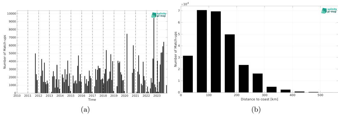
Figure 2: Number of match-ups between TSG (SAMOS) and SMAP SSS L4 OI v3 - Monthly (ESR) SSS as a function of time (a) and as function of the distance to coast (b) over the Mississippi river plume Pi-MEP region and for the full satellite product period.
