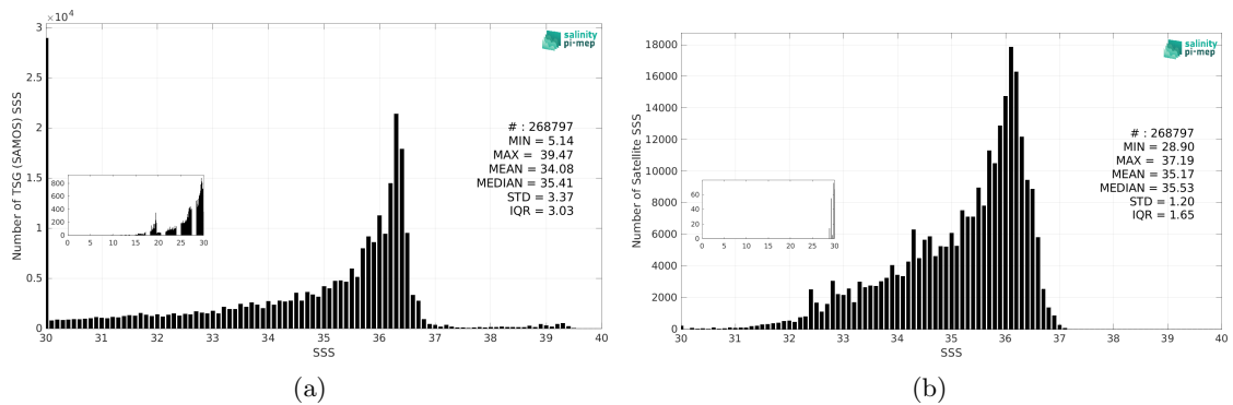
Figure 3: Histograms of SSS from TSG (SAMOS) (a) and SMAP SSS L4 OI v3 - Monthly (ESR) (b) considering all match-up pairs per bins of 0.1 over the Mississippi river plume Pi-MEP region and for the full satellite product period.
