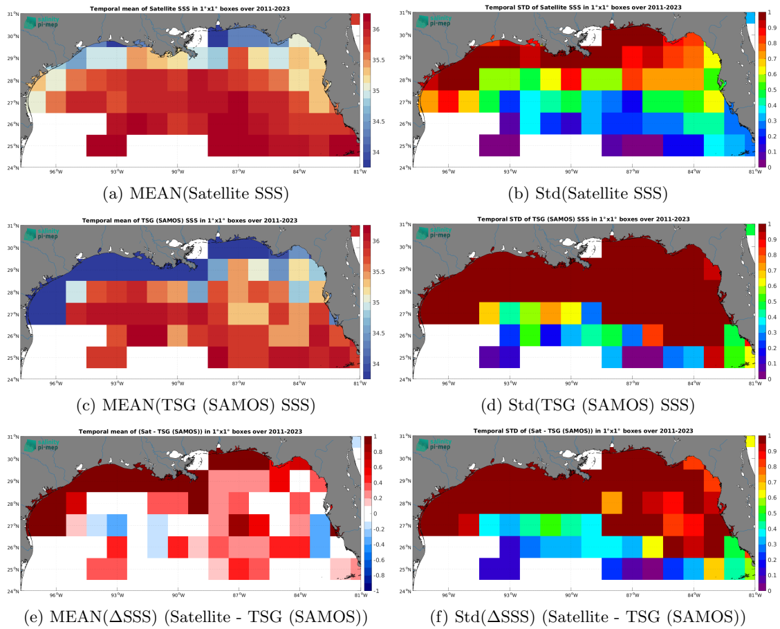
Figure 7: Temporal mean (left) and Std (right) of SSS from SMAP SSS L4 OI v3 - Monthly (ESR) (top), TSG (SAMOS) (middle), and of \Delta SSS (Satellite - TSG (SAMOS)). Only match-up pairs are used to generate these maps.
