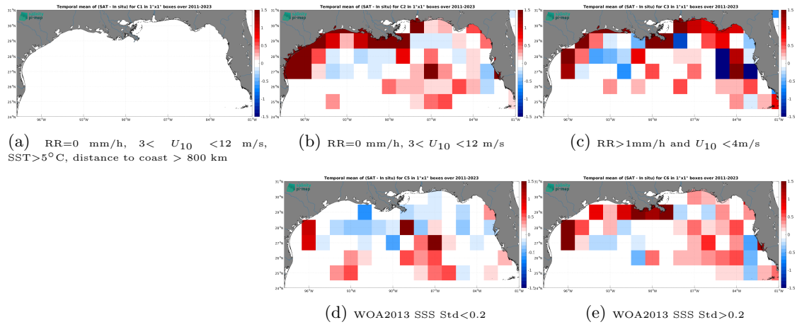
Figure 14: Temporal mean gridded over spatial boxes of size 1^\circ \times 1^\circ of \Delta SSS (SMAP SSS L4 OI v3 - Daily (ESR) - TSG (SAMOS)) for 5 different subdatasets corresponding to: RR=0 mm/h, 3 < U_{10} < 12 m/s, SST > 5^\circ C , distance to coast > 800 km (a), RR=0 mm/h, 3 < U_{10} < 12 m/s (b), RR > 1 mm/h and U_{10} < 4 m/s (c), WOA2013 SSS Std < 0.2 (d), WOA2013 SSS Std > 0.2 (e).
