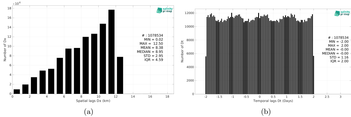
Figure 6: Histograms of the spatial (a) and temporal (b) lags between the location/time of the TSG (SAMOS) measurement and the date of the corresponding SMAP SSS L4 OI v3 - Daily (ESR) SSS pixel.
