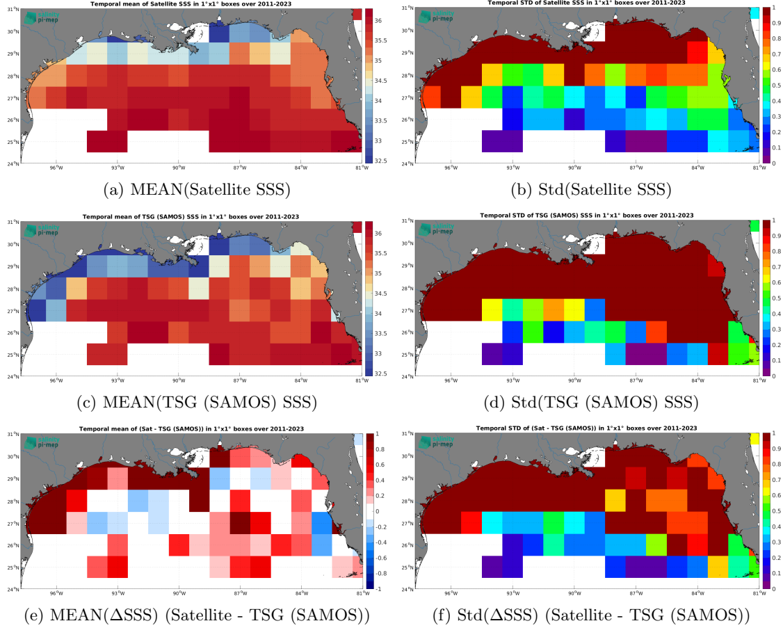
Figure 7: Temporal mean (left) and Std (right) of SSS from SMAP SSS L4 OI v3 - Daily (ESR) (top), TSG (SAMOS) (middle), and of \Delta\text{SSS} (Satellite - TSG (SAMOS)). Only match-up pairs are used to generate these maps.
