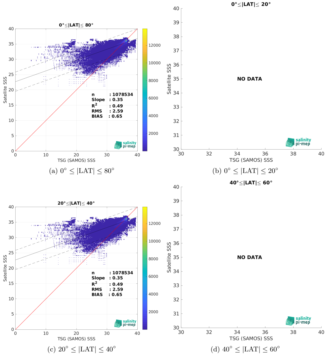
Figure 10: Contour maps of the concentration of SMAP SSS L4 OI v3 - Daily (ESR) SSS (y-axis) versus TSG (SAMOS) SSS (x-axis) at match-up pairs for different latitude bands. For each plot, the red line shows x=y . The black thin and dashed lines indicate a linear fit through the data cloud and the \pm 95\% confidence levels, respectively. The number match-up pairs n , the slope and R^2 coefficient of the linear fit, the root mean square (RMS) and the mean bias between satellite and in situ data are indicated for each latitude band in each plots.
