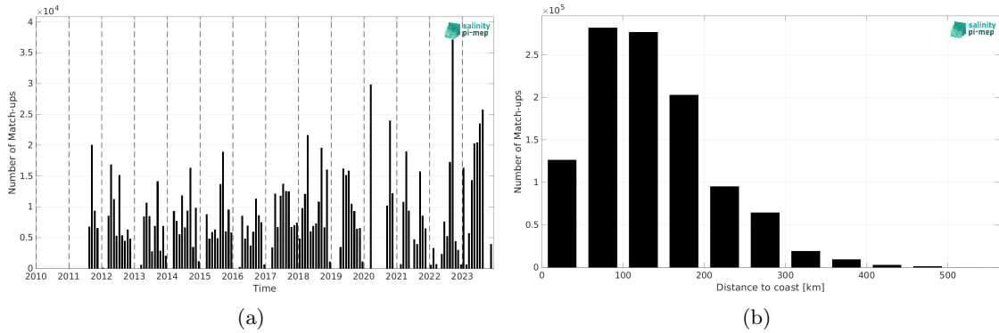
Figure 2: Number of match-ups between TSG (SAMOS) and SMAP SSS L4 OI v3 - Daily (ESR) SSS as a function of time (a) and as function of the distance to coast (b) over the Mississippi river plume Pi-MEP region and for the full satellite product period.
