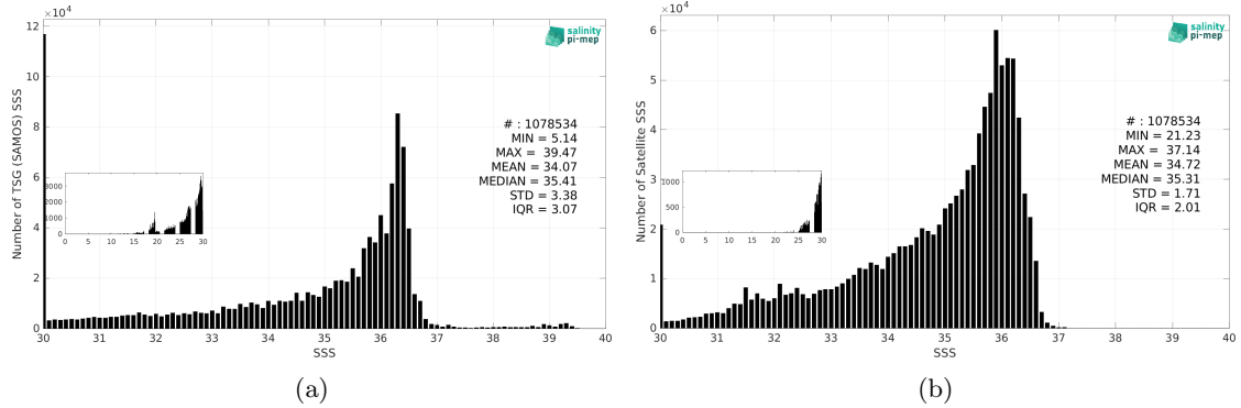
Figure 3: Histograms of SSS from TSG (SAMOS) (a) and SMAP SSS L4 OI v3 - Daily (ESR) (b) considering all match-up pairs per bins of 0.1 over the Mississippi river plume Pi-MEP region and for the full satellite product period.
