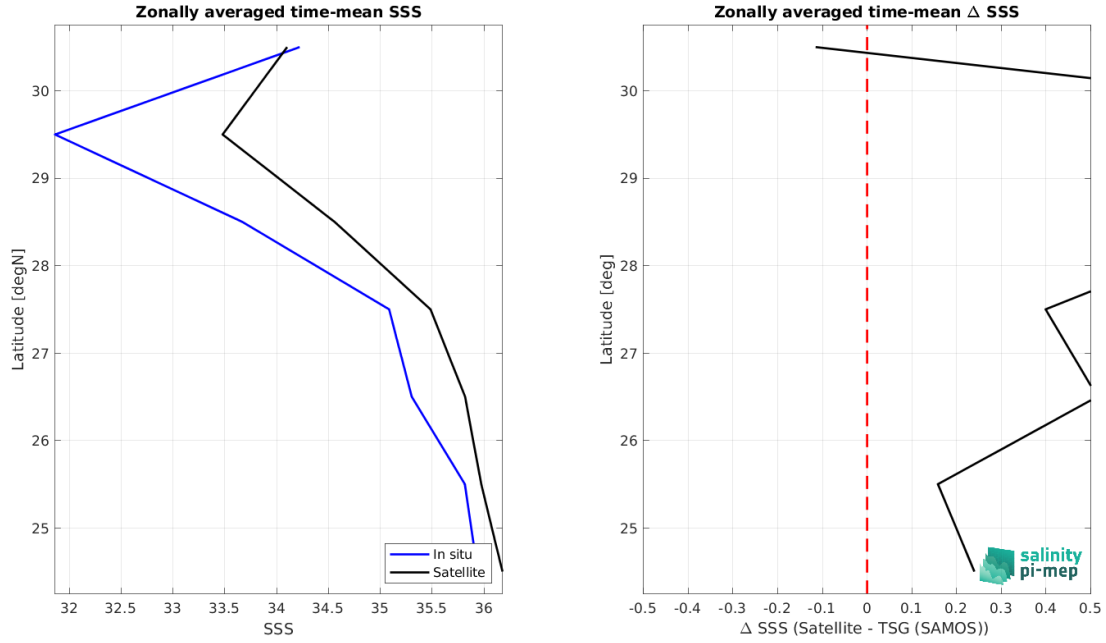
Figure 9: Left panel: Zonal mean SSS from SMAP SSS L4 OI v3 - Daily (ESR) satellite product (black) and from TSG (SAMOS) (blue). Right panel: Zonal mean of \Delta SSS (Satellite - TSG (SAMOS)) for all the collected Pi-MEP match-up pairs estimated over the full satellite product period.
