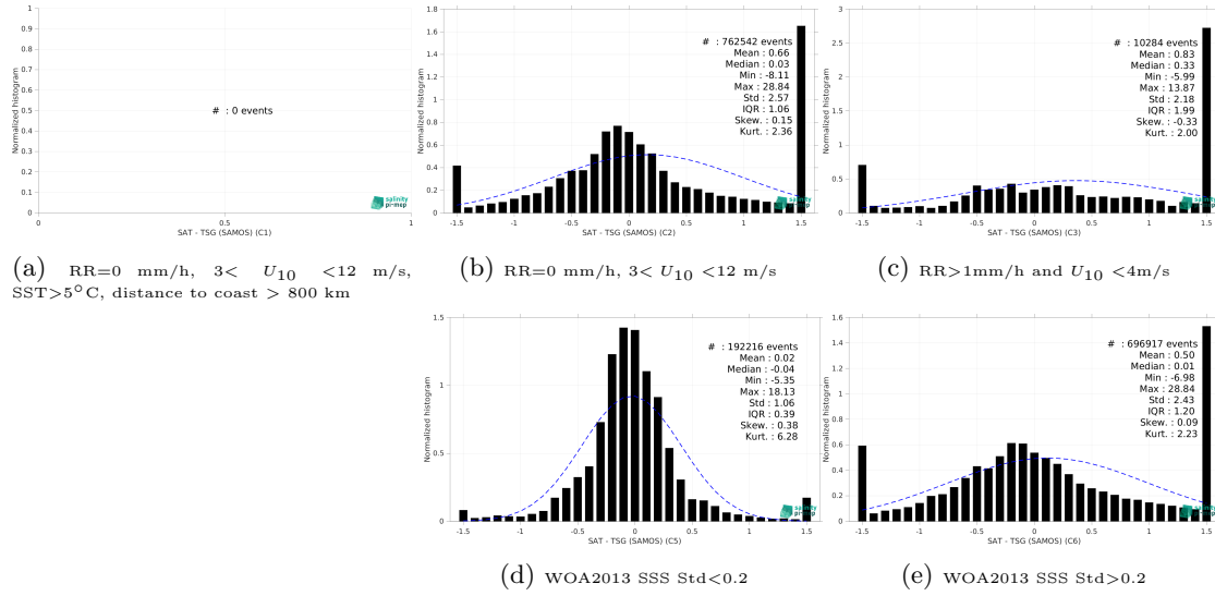
Figure 15: Normalized histogram of \Delta SSS (SMAP SSS L4 OI v3 - Daily (ESR) - TSG (SAMOS)) for 5 different subdatasets corresponding to: RR=0 mm/h, 3 < U_{10} < 12 m/s, SST>5°C, distance to coast > 800 km (a), RR=0 mm/h, 3 < U_{10} < 12 m/s (b), RR>1mm/h and U_{10} < 4 m/s (c), WOA2013 SSS Std<0.2 (d), WOA2013 SSS Std>0.2 (e).
