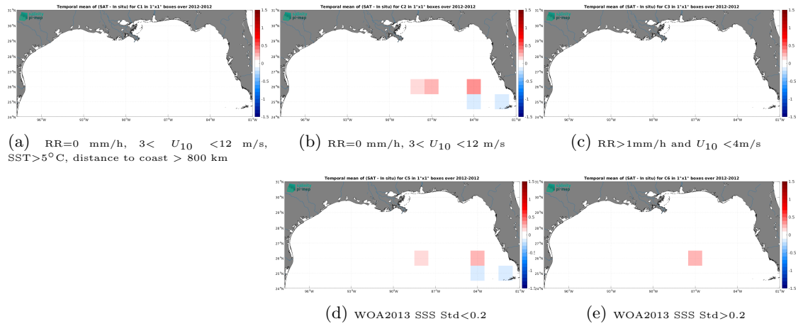
Figure 14: Temporal mean gridded over spatial boxes of size 1^\circ \times 1^\circ of \Delta SSS (SMAP SSS L4 OI v3 - Daily (ESR) - TSG (GOSUD-Sailing-ship)) for 5 different subdatasets corresponding to: RR=0 mm/h, 3 < U_{10} < 12 m/s, SST > 5^\circ C , distance to coast > 800 km (a), RR=0 mm/h, 3 < U_{10} < 12 m/s (b), RR > 1 mm/h and U_{10} < 4 m/s (c), WOA2013 SSS Std < 0.2 (d), WOA2013 SSS Std > 0.2 (e).
