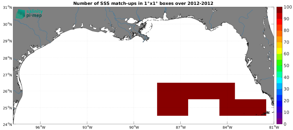
Figure 5: Number of SSS match-ups between TSG (GOSUD-Sailing-ship) SSS and the SMAP SSS L4 OI v3 - Daily (ESR) SSS product for the Mississippi river plume Pi-MEP region over 1^\circ \times 1^\circ boxes and for the full satellite product period.
