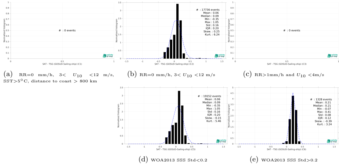
Figure 15: Normalized histogram of \Delta SSS (SMAP SSS L4 OI v3 - Daily (ESR) - TSG (GOSUD-Sailing-ship)) for 5 different subdatasets corresponding to: RR=0 mm/h, 3 < U_{10} < 12 m/s, SST>5°C, distance to coast > 800 km (a), RR=0 mm/h, 3 < U_{10} < 12 m/s (b), RR>1mm/h and U_{10} < 4 m/s (c), WOA2013 SSS Std<0.2 (d), WOA2013 SSS Std>0.2 (e).
