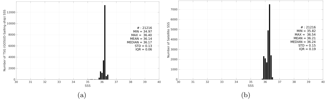
Figure 3: Histograms of SSS from TSG (GOSUD-Sailing-ship) (a) and SMAP SSS L4 OI v3 - Daily (ESR) (b) considering all match-up pairs per bins of 0.1 over the Mississippi river plume Pi-MEP region and for the full satellite product period.
