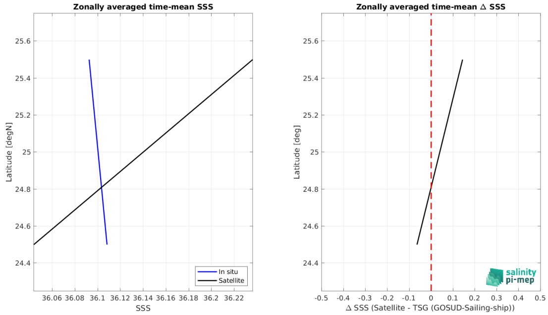
Figure 9: Left panel: Zonal mean SSS from SMAP SSS L4 OI v3 - Daily (ESR) satellite product (black) and from TSG (GOSUD-Sailing-ship) (blue). Right panel: Zonal mean of \Delta SSS (Satellite - TSG (GOSUD-Sailing-ship)) for all the collected Pi-MEP match-up pairs estimated over the full satellite product period.
