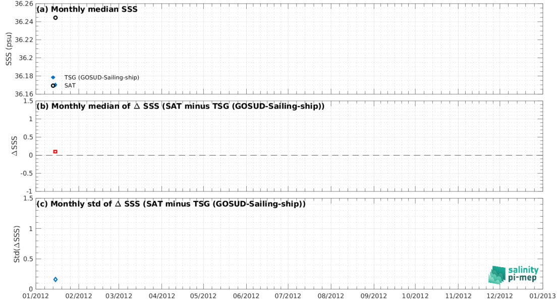
Figure 8: Time series of the monthly median SSS (top), median of \Delta SSS (Satellite - TSG (GOSUD-Sailing-ship)) and Std of \Delta SSS (Satellite - TSG (GOSUD-Sailing-ship)) over the Mississippi river plume Pi-MEP region considering all match-ups collected by the Pi-MEP.
