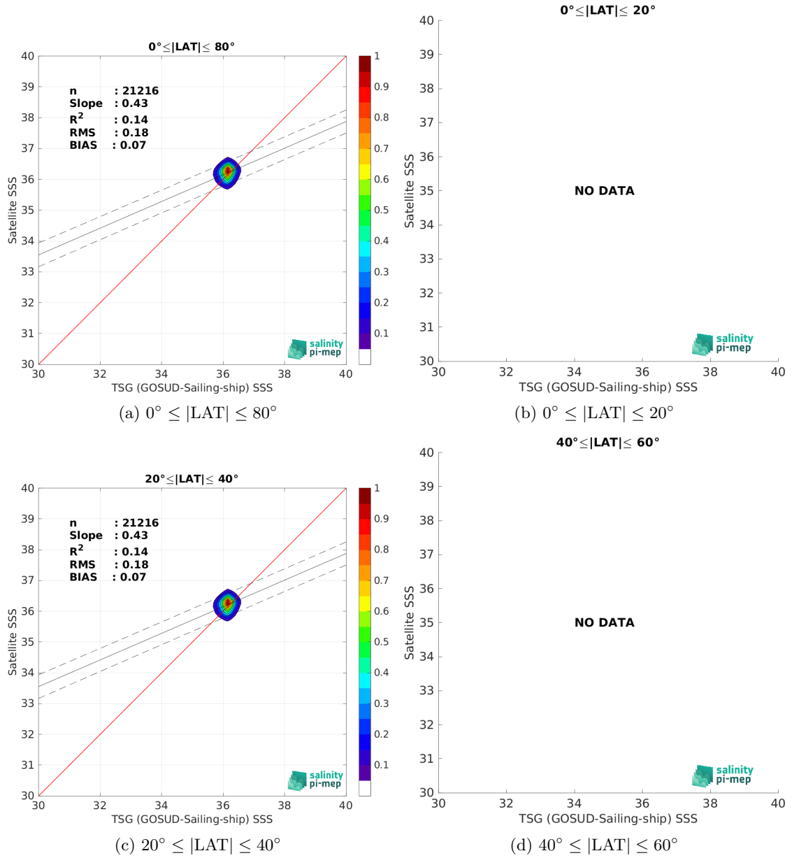
Figure 10: Contour maps of the concentration of SMAP SSS L4 OI v3 - Daily (ESR) SSS (y-axis) versus TSG (GOSUD-Sailing-ship) SSS (x-axis) at match-up pairs for different latitude bands. For each plot, the red line shows x=y . The black thin and dashed lines indicate a linear fit through the data cloud and the \pm 95\% confidence levels, respectively. The number match-up pairs n , the slope and R^2 coefficient of the linear fit, the root mean square (RMS) and the mean bias between satellite and in situ data are indicated for each latitude band in each plots.
