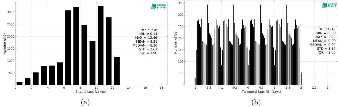
Figure 6: Histograms of the spatial (a) and temporal (b) lags between the location/time of the TSG (GOSUD-Sailing-ship) measurement and the date of the corresponding SMAP SSS L4 OI v3 - Daily (ESR) SSS pixel.
