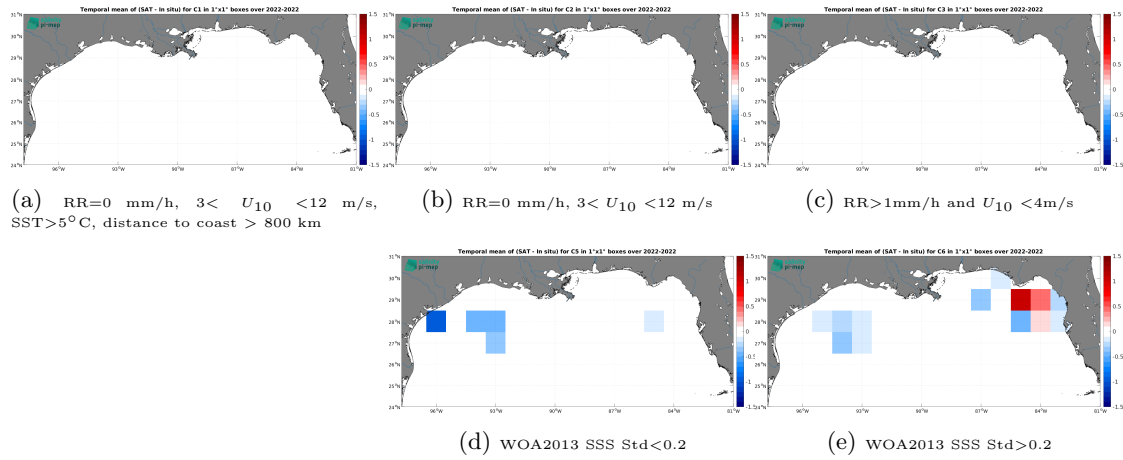
Figure 14: Temporal mean gridded over spatial boxes of size 1^\circ \times 1^\circ of \Delta SSS (SMAP SSS L4 OI v3 - Daily (ESR) - Saildrone) for 5 different subdatasets corresponding to: RR=0 mm/h, 3 < U_{10} < 12 m/s, SST > 5^\circ C , distance to coast > 800 km (a), RR=0 mm/h, 3 < U_{10} < 12 m/s (b), RR > 1 mm/h and U_{10} < 4 m/s (c), WOA2013 SSS Std < 0.2 (d), WOA2013 SSS Std > 0.2 (e).
