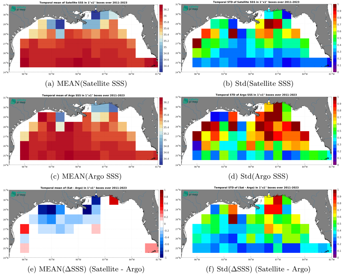
Figure 7: Temporal mean (left) and Std (right) of SSS from SMAP SSS L4 OI v3 - Daily (ESR) (top), Argo (middle), and of \Delta SSS (Satellite - Argo). Only match-up pairs are used to generate these maps.
