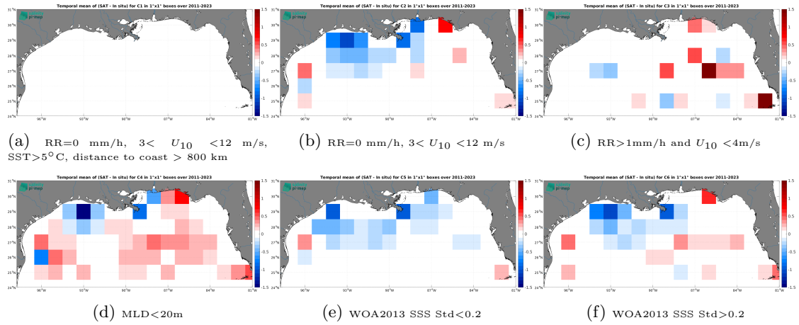
Figure 14: Temporal mean gridded over spatial boxes of size 1^\circ \times 1^\circ of \Delta SSS (SMAP SSS L4 OI v3 - Daily (ESR) - Argo) for 6 different subdatasets corresponding to:RR=0 mm/h, 3 < U_{10} < 12 m/s, SST >5^\circ\text{C} , distance to coast > 800 km (a), RR=0 mm/h, 3 < U_{10} < 12 m/s (b), RR >1 mm/h and U_{10} < 4 m/s (c),MLD <20 m (d),WOA2013 SSS Std <0.2 (e),WOA2013 SSS Std >0.2 (f).
