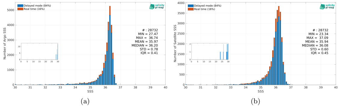
Figure 3: Histograms of SSS from Argo (a) and SMAP SSS L4 OI v3 - Daily (ESR) (b) considering all match-up pairs per bins of 0.1 over the Mississippi river plume Pi-MEP region and for the full satellite product period.
