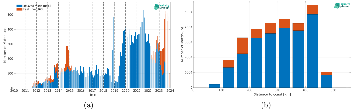
Figure 2: Number of match-ups between Argo and SMAP SSS L4 OI v3 - Daily (ESR) SSS as a function of time (a) and as function of the distance to coast (b) over the Mississippi river plume Pi-MEP region and for the full satellite product period.
