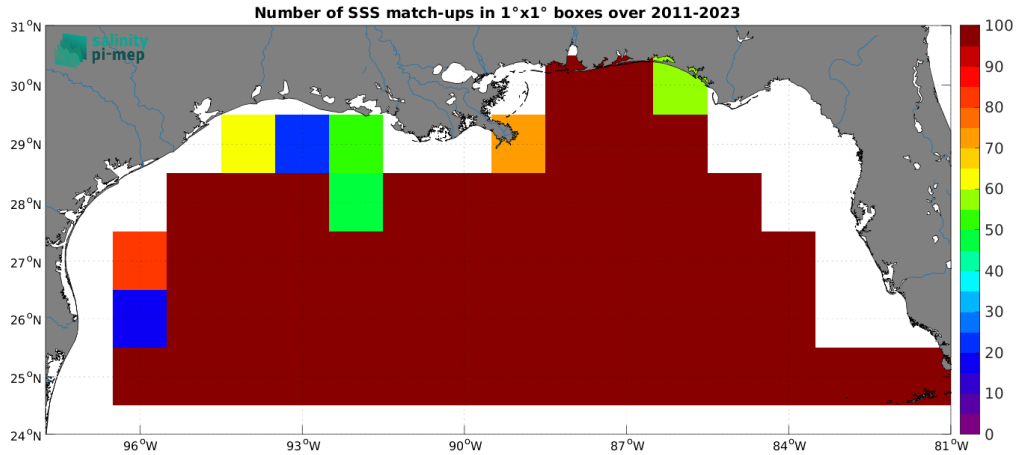
Figure 5: Number of SSS match-ups between Argo SSS and the SMAP SSS L4 OI v3 - Daily (ESR) SSS product for the Mississippi river plume Pi-MEP region over 1^\circ \times 1^\circ boxes and for the full satellite product period.
