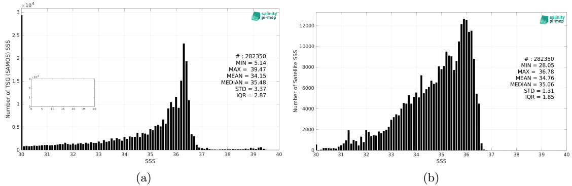
Figure 2: Histograms of SSS from TSG (SAMOS) (a) and SMAP SSS L4 OI v2 - 7 Days (ESR) (b) considering all match-up pairs per bins of 0.1 over the Mississippi river plume Pi-MEP region and for the full satellite product period.
