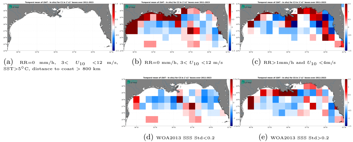
Figure 12: Temporal mean gridded over spatial boxes of size 1^{\circ}\times 1^{\circ} of \Delta\text{SSS} (SMAP SSS L4 OI v2 - 7 Days (ESR) - TSG (SAMOS)) for 5 different subdatasets corresponding to:RR=0 mm/h, 3 < U_{10} < 12 m/s, SST > 5^{\circ}\text{C} , distance to coast > 800 km (a), RR=0 mm/h, 3 < U_{10} < 12 m/s (b), RR > 1 mm/h and U_{10} < 4 m/s (c), WOA2013 SSS Std < 0.2 (d), WOA2013 SSS Std > 0.2 (e).
