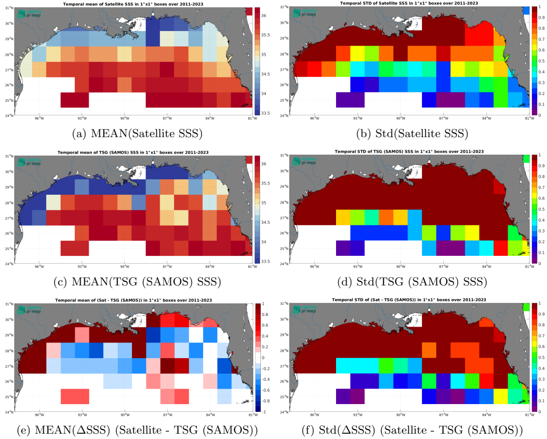
Figure 6: Temporal mean (left) and Std (right) of SSS from SMAP SSS L4 OI v2 - 7 Days (ESR) (top), TSG (SAMOS) (middle), and of \Delta\text{SSS} (Satellite - TSG (SAMOS)). Only match-up pairs are used to generate these maps.
