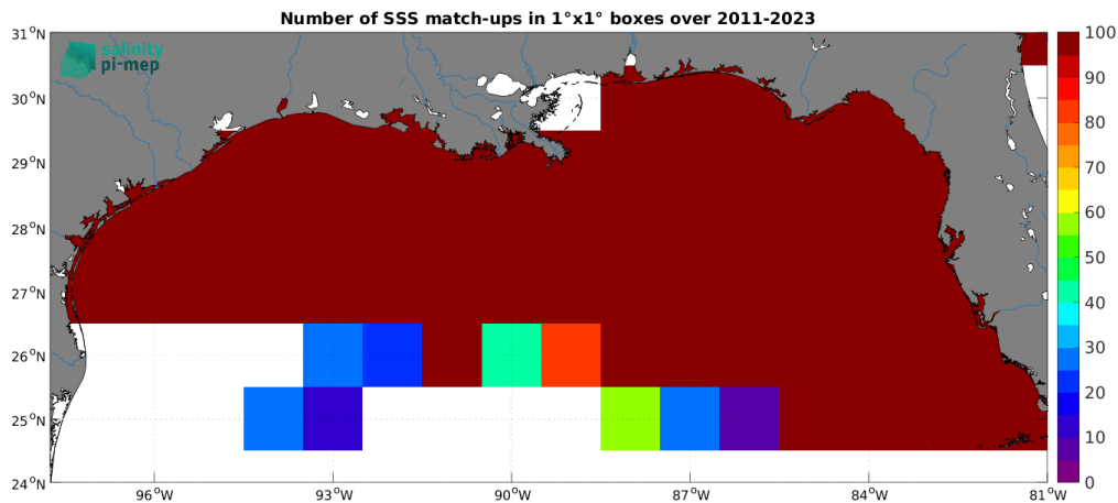
Figure 4: Number of SSS match-ups between TSG (SAMOS) SSS and the SMAP SSS L4 OI v2 - 7 Days (ESR) SSS product for the Mississippi river plume Pi-MEP region over 1^\circ \times 1^\circ boxes and for the full satellite product period.
