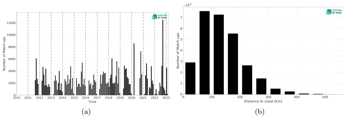
Figure 1: Number of match-ups between TSG (SAMOS) and SMAP SSS L4 OI v2 - 7 Days (ESR) SSS as a function of time (a) and as function of the distance to coast (b) over the Mississippi river plume Pi-MEP region and for the full satellite product period.
