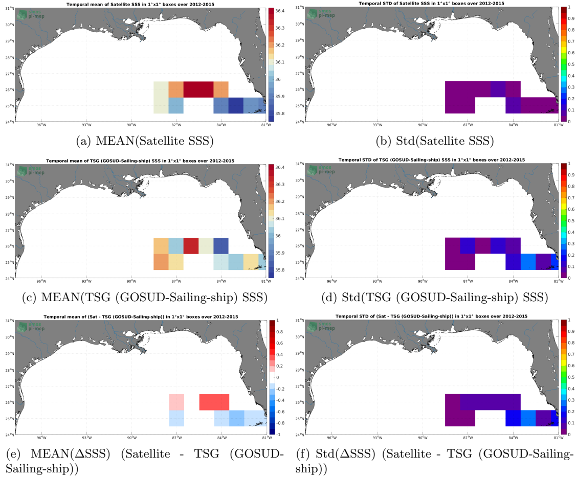
Figure 6: Temporal mean (left) and Std (right) of SSS from SMAP SSS L4 OI v2 - 7 Days (ESR) (top), TSG (GOSUD-Sailing-ship) (middle), and of \Delta\text{SSS} (Satellite - TSG (GOSUD-Sailing-ship)). Only match-up pairs are used to generate these maps.
