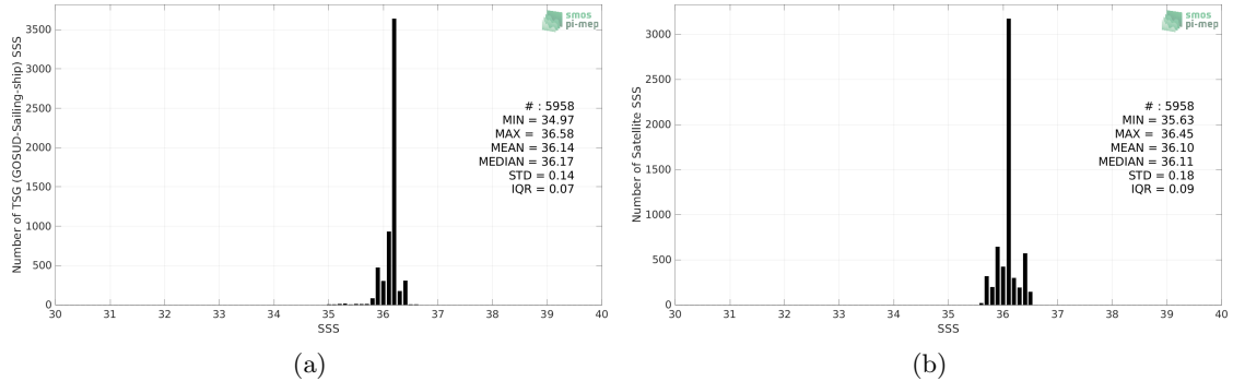
Figure 2: Histograms of SSS from TSG (GOSUD-Sailing-ship) (a) and SMAP SSS L4 OI v2 - 7 Days (ESR) (b) considering all match-up pairs per bins of 0.1 over the Mississippi river plume Pi-MEP region and for the full satellite product period.
