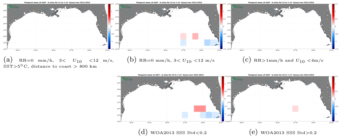
Figure 12: Temporal mean gridded over spatial boxes of size 1^{\circ}\times 1^{\circ} of \Delta SSS (SMAP SSS L4 OI v2 - 7 Days (ESR) - TSG (GOSUD-Sailing-ship)) for 5 different subdatasets corresponding to:RR=0 mm/h, 3 < U_{10} < 12 m/s, SST >5^{\circ}\text{C} , distance to coast > 800 km (a), RR=0 mm/h, 3 < U_{10} < 12 m/s (b), RR >1 mm/h and U_{10} < 4 m/s (c), WOA2013 SSS Std <0.2 (d), WOA2013 SSS Std >0.2 (e).
