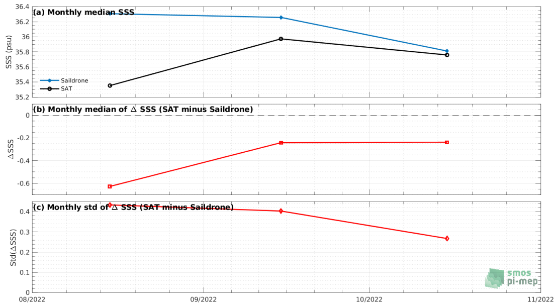
Figure 7: Time series of the monthly median SSS (top), median of \Delta SSS (Satellite - Sairdrones) and Std of \Delta SSS (Satellite - Sairdrones) over the Mississippi river plume Pi-MEP region considering all match-ups collected by the Pi-MEP.
