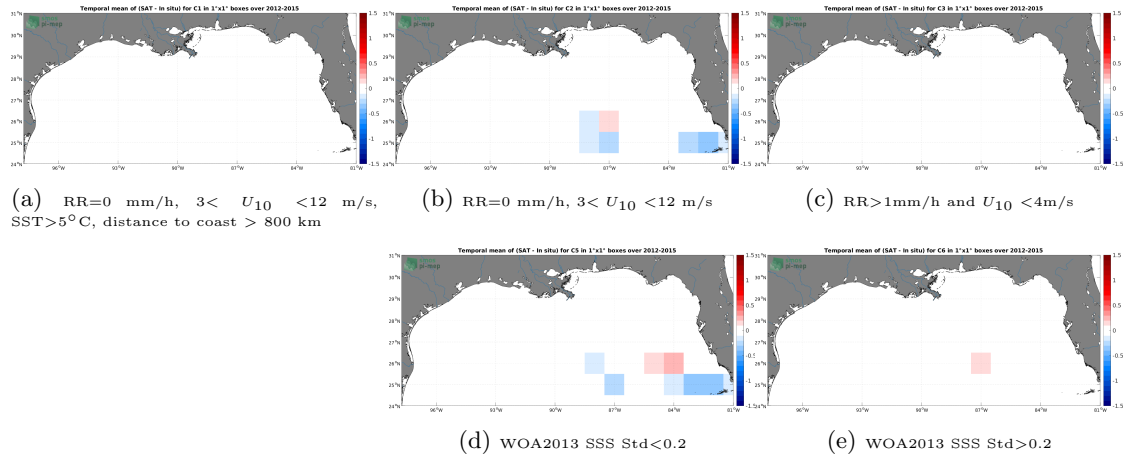
Figure 12: Temporal mean gridded over spatial boxes of size 1^\circ \times 1^\circ of \Delta SSS (SMAP SSS L4 OI v2 - Monthly (IPRC) - TSG (GOSUD-Sailing-ship)) for 5 different subdatasets corresponding to:RR=0 mm/h, 3 < U_{10} < 12 m/s, SST >5^\circ\text{C} , distance to coast > 800 km (a), RR=0 mm/h, 3 < U_{10} < 12 m/s (b), RR >1 mm/h and U_{10} < 4 m/s (c), WOA2013 SSS Std <0.2 (d), WOA2013 SSS Std >0.2 (e).
