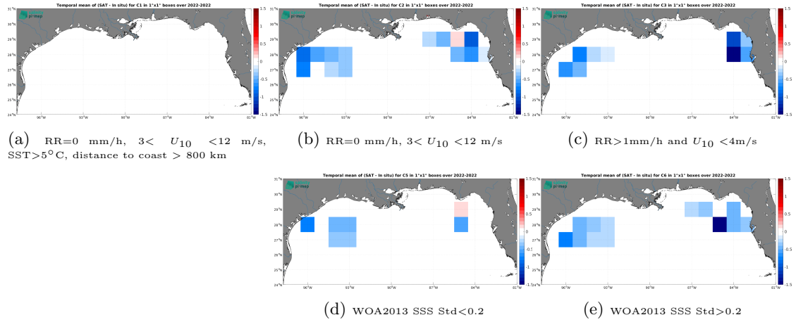
Figure 12: Temporal mean gridded over spatial boxes of size 1^{\circ}\times 1^{\circ} of \Delta\text{SSS} (SMAP SSS L4 OI v2 - Monthly (IPRC) - Saildrone) for 5 different subdatasets corresponding to:RR=0 mm/h, 3 < U_{10} < 12 m/s, SST > 5^{\circ}\text{C} , distance to coast > 800 km (a), RR=0 mm/h, 3 < U_{10} < 12 m/s (b), RR > 1 mm/h and U_{10} < 4 m/s (c), WOA2013 SSS Std < 0.2 (d), WOA2013 SSS Std > 0.2 (e).
