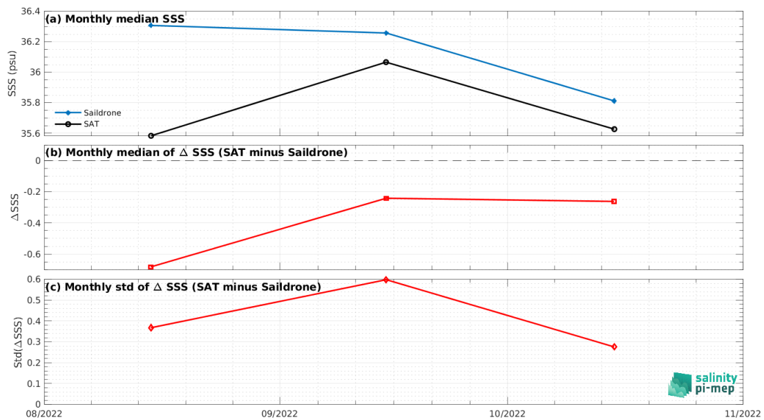
Figure 7: Time series of the monthly median SSS (top), median of \Delta SSS (Satellite - Saildrone) and Std of \Delta SSS (Satellite - Saildrone) over the Mississippi river plume Pi-MEP region considering all match-ups collected by the Pi-MEP.
