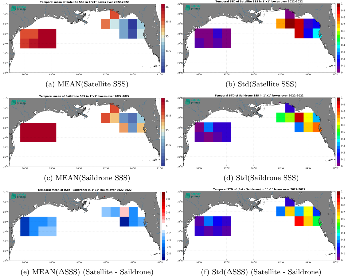
Figure 6: Temporal mean (left) and Std (right) of SSS from SMAP SSS L4 OI v2 - Monthly (IPRC) (top), Sairdron (middle), and of \Delta SSS (Satellite - Sairdron). Only match-up pairs are used to generate these maps.
