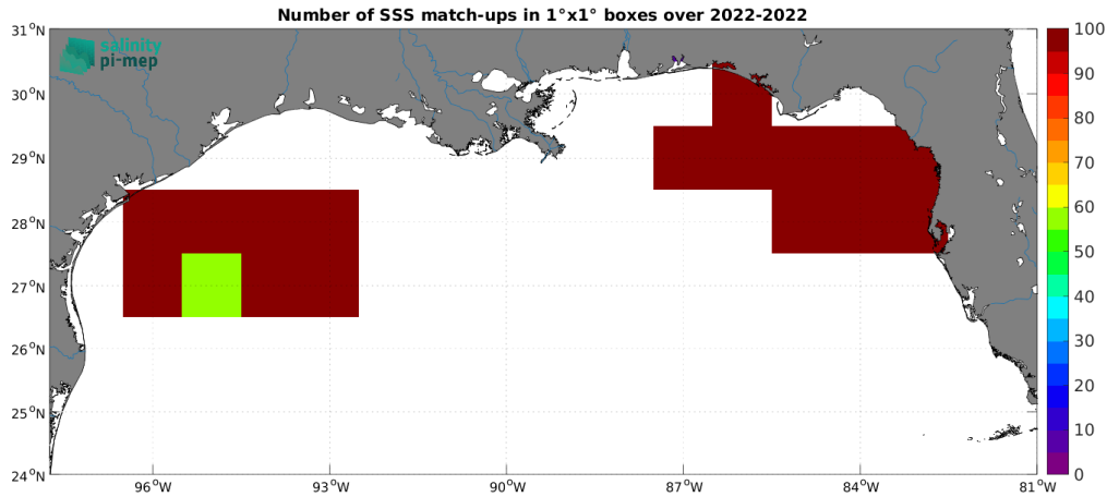
Figure 4: Number of SSS match-ups between Saildrone SSS and the SMAP SSS L4 OI v2 - Monthly (IPRC) SSS product for the Mississippi river plume Pi-MEP region over 1^\circ \times 1^\circ boxes and for the full satellite product period.
