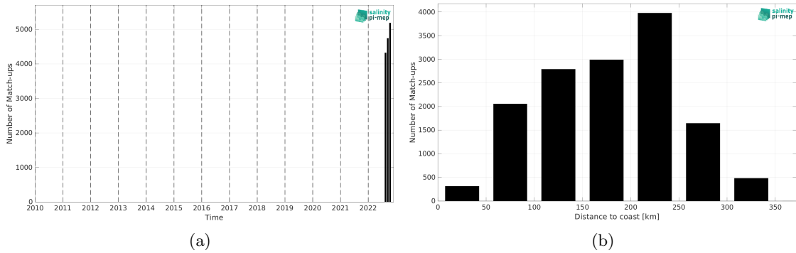
Figure 1: Number of match-ups between Saildrone and SMAP SSS L4 OI v2 - Monthly (IPRC) SSS as a function of time (a) and as function of the distance to coast (b) over the Mississippi river plume Pi-MEP region and for the full satellite product period.
