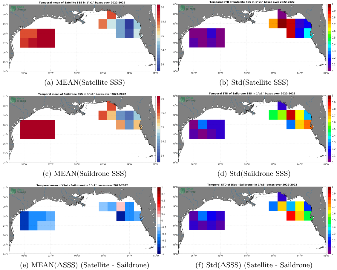
Figure 6: Temporal mean (left) and Std (right) of SSS from SMAP SSS L4 OI v2 - Monthly (IPRC) (top), Sairdron (middle), and of \Delta\text{SSS} (Satellite - Sairdron). Only match-up pairs are used to generate these maps.
