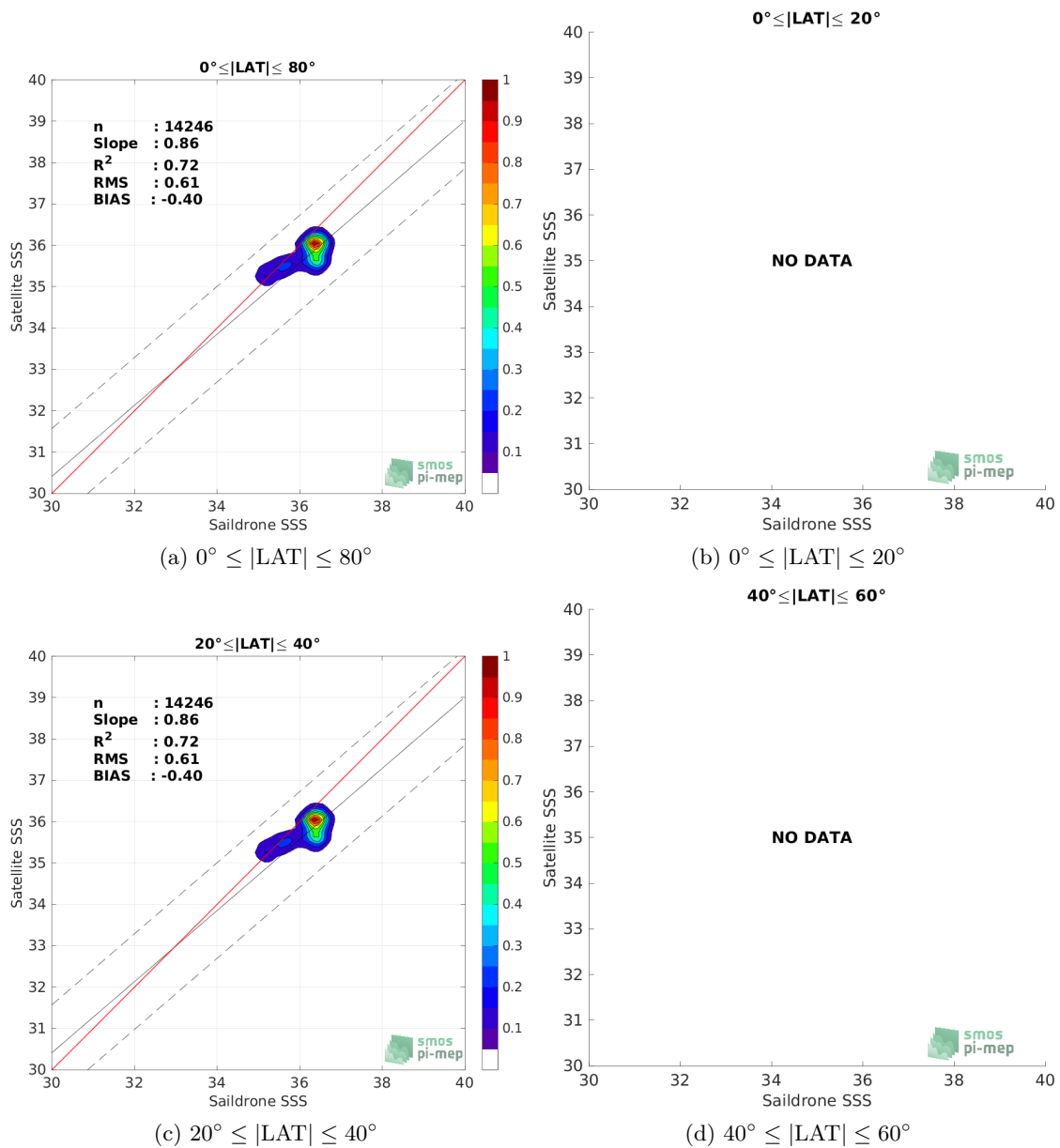
Figure 9: Contour maps of the concentration of SMAP SSS L4 OI v2 - Monthly (IPRC) SSS (y-axis) versus Saïldrone SSS (x-axis) at match-up pairs for different latitude bands. For each plot, the red line shows x=y . The black thin and dashed lines indicate a linear fit through the data cloud and the \pm 95\% confidence levels, respectively. The number match-up pairs n , the slope and R^2 coefficient of the linear fit, the root mean square (RMS) and the mean bias between satellite and in situ data are indicated for each latitude band in each plots.
