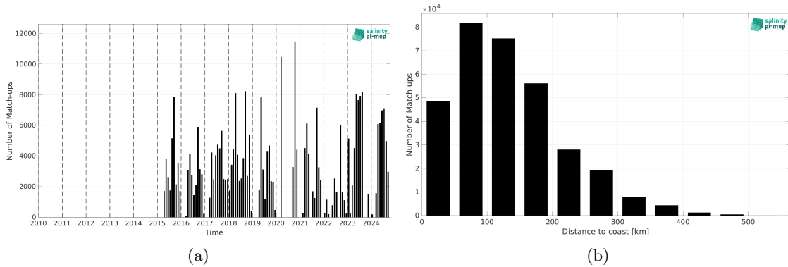
Figure 2: Number of match-ups between TSG (SAMOS) and SMAP SSS L3 v6 - 8-Day running (RSS) SSS as a function of time (a) and as function of the distance to coast (b) over the Mississippi river plume Pi-MEP region and for the full satellite product period.
