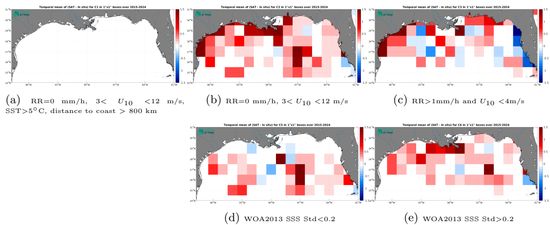
Figure 14: Temporal mean gridded over spatial boxes of size 1^\circ \times 1^\circ of \Delta SSS (SMAP SSS L3 v6 - 8-Day running (RSS) - TSG (SAMOS)) for 5 different subdatasets corresponding to:RR=0 mm/h, 3 < U_{10} < 12 m/s, SST >5^\circ C, distance to coast > 800 km (a), RR=0 mm/h, 3 < U_{10} < 12 m/s (b), RR >1 mm/h and U_{10} < 4 m/s (c), WOA2013 SSS Std <0.2 (d), WOA2013 SSS Std >0.2 (e).
