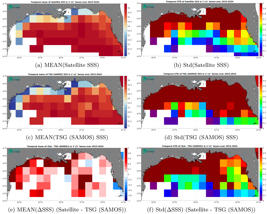
Figure 7: Temporal mean (left) and Std (right) of SSS from SMAP SSS L3 v6 - 8-Day running (RSS) (top), TSG (SAMOS) (middle), and of \Delta\text{SSS} (Satellite - TSG (SAMOS)). Only match-up pairs are used to generate these maps.
