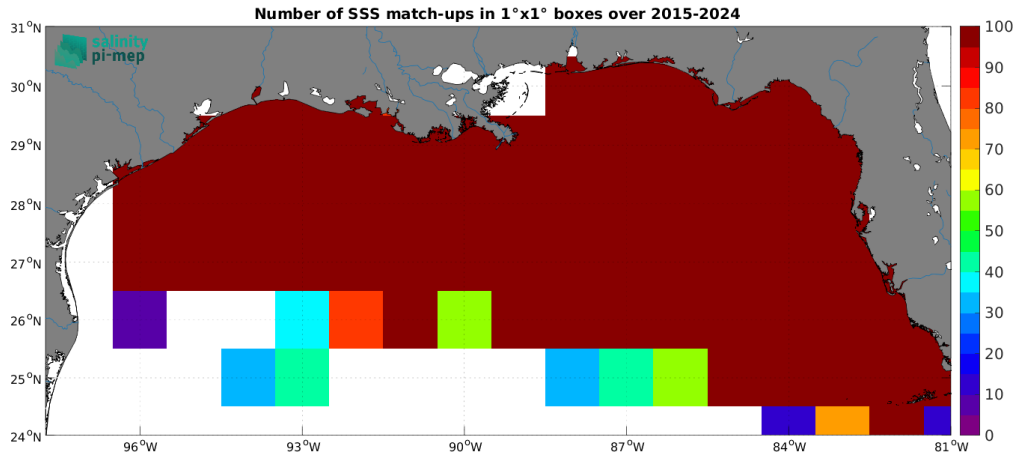
Figure 5: Number of SSS match-ups between TSG (SAMOS) SSS and the SMAP SSS L3 v6 - 8-Day running (RSS) SSS product for the Mississippi river plume Pi-MEP region over 1^\circ \times 1^\circ boxes and for the full satellite product period.
