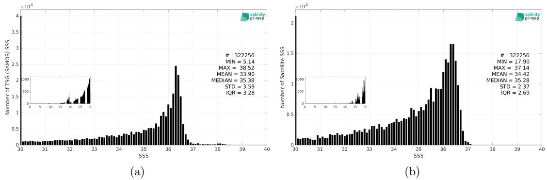
Figure 3: Histograms of SSS from TSG (SAMOS) (a) and SMAP SSS L3 v6 - 8-Day running (RSS) (b) considering all match-up pairs per bins of 0.1 over the Mississippi river plume Pi-MEP region and for the full satellite product period.
