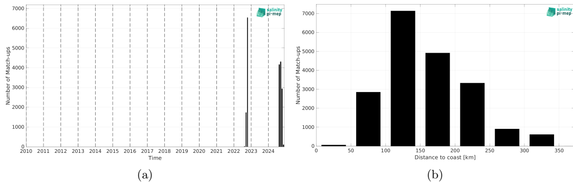
Figure 2: Number of match-ups between Saildrone and SMAP SSS L3 v6 - 8-Day running (RSS) SSS as a function of time (a) and as function of the distance to coast (b) over the Mississippi river plume Pi-MEP region and for the full satellite product period.
