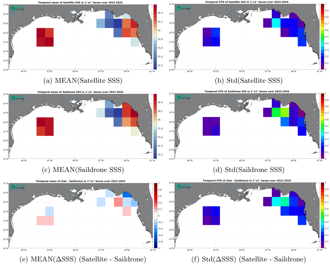
Figure 7: Temporal mean (left) and Std (right) of SSS from SMAP SSS L3 v6 - 8-Day running (RSS) (top), Saildrone (middle), and of \Delta\text{SSS} (Satellite - Saildrone). Only match-up pairs are used to generate these maps.
