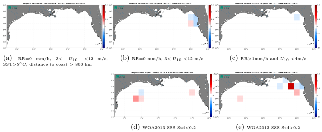
Figure 14: Temporal mean gridded over spatial boxes of size 1^\circ \times 1^\circ of \Delta SSS (SMAP SSS L3 v6 - 8-Day running (RSS) - Sailability) for 5 different subdatasets corresponding to: RR=0 mm/h, 3 < U_{10} < 12 m/s, SST > 5°C, distance to coast > 800 km (a), RR=0 mm/h, 3 < U_{10} < 12 m/s (b), RR > 1mm/h and U_{10} < 4 m/s (c), WOA2013 SSS Std < 0.2 (d), WOA2013 SSS Std > 0.2 (e).
