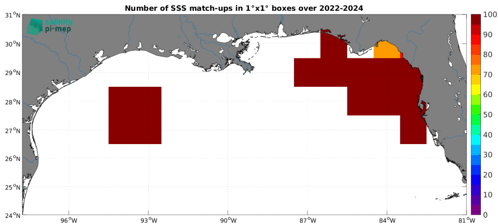
Figure 5: Number of SSS match-ups between Saildrone SSS and the SMAP SSS L3 v6 - 8-Day running (RSS) SSS product for the Mississippi river plume Pi-MEP region over 1^\circ \times 1^\circ boxes and for the full satellite product period.
